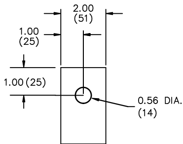
TERMINAL 0.25 X 2.00 COPPER
