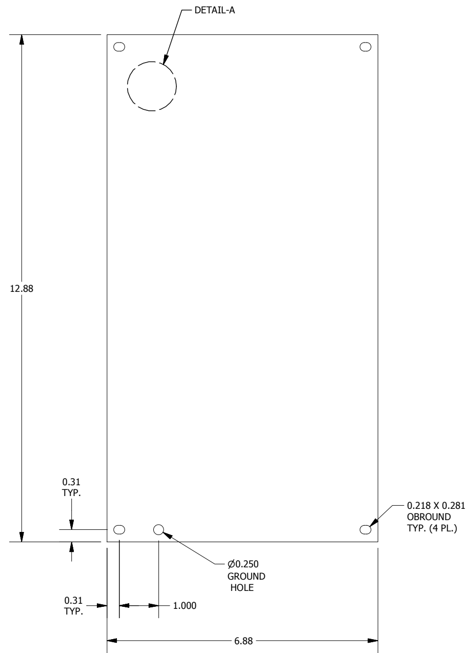
FRONT VIEW
