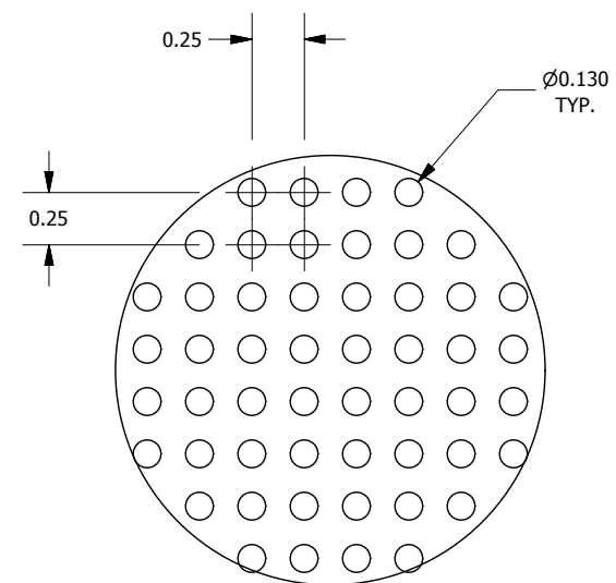
DETAIL-A (PERFORATED DETAIL)
