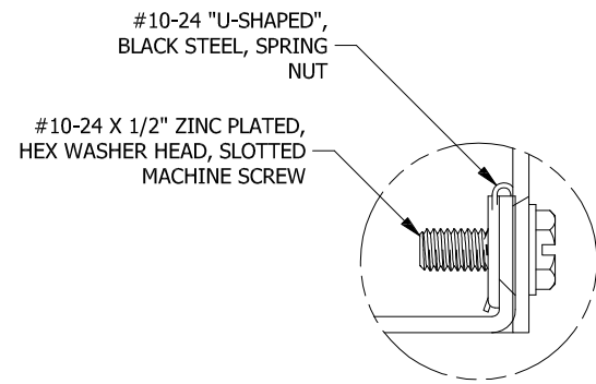
DETAIL A (5 PL.) (LID ATTACHMENT DETAIL)
