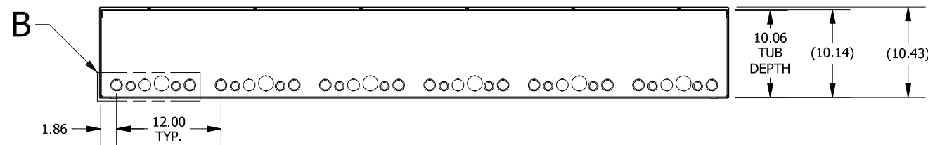
BOTTOM VIEW
