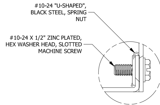
DETAIL A (6 PL.) (LID ATTACHMENT DETAIL)
