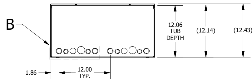
BOTTOM VIEW
