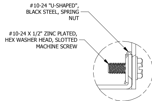
DETAIL A (2 PL.) (LID ATTACHMENT DETAIL)
