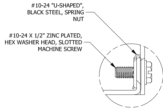
DETAIL A (2 PL.) (LID ATTACHMENT DETAIL)
