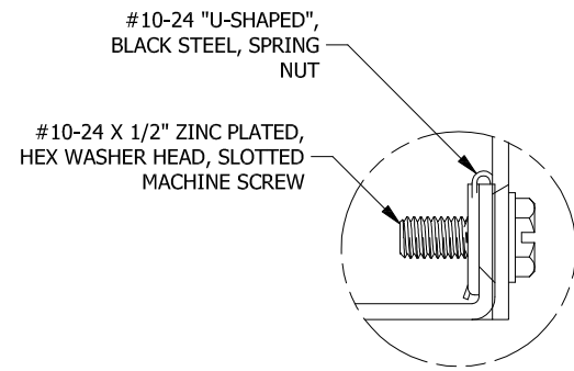
DETAIL A (3 PL.) (LID ATTACHMENT DETAIL)
