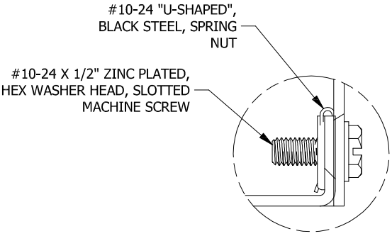
DETAIL A (3 PL.) (LID ATTACHMENT DETAIL)
