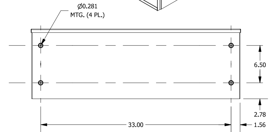
BACK VIEW
