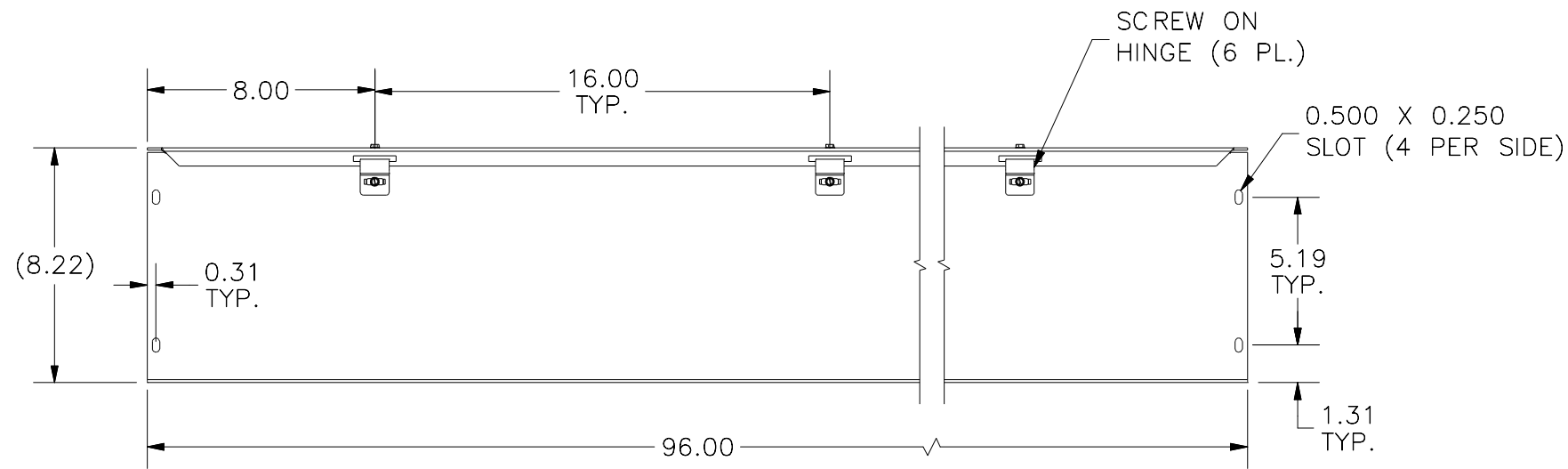
FRONT VIEW
