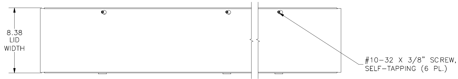
TOP VIEW
