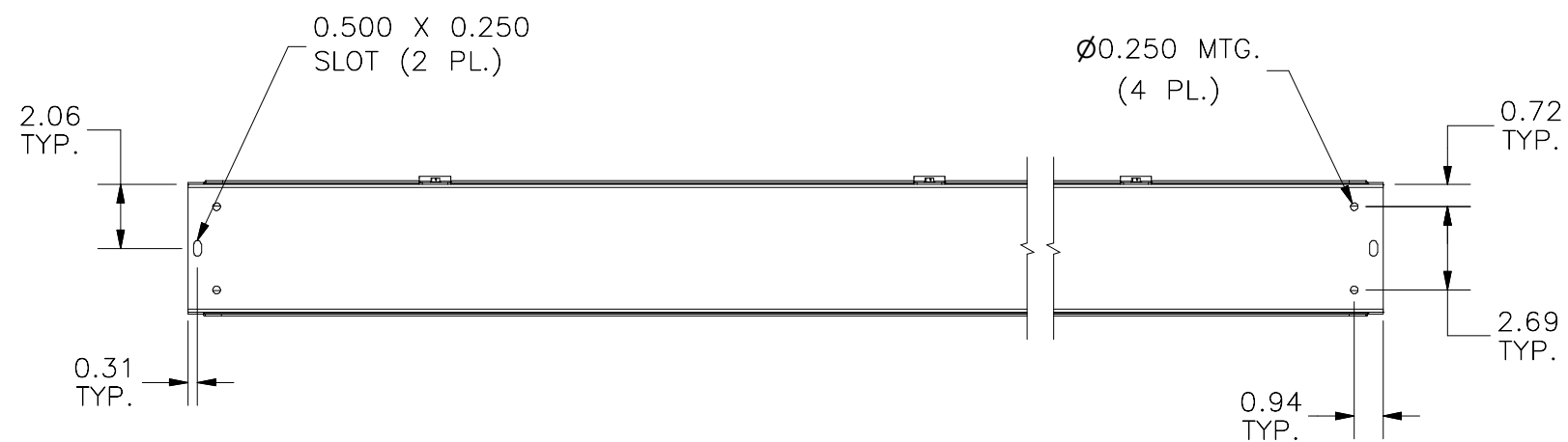
BOTTOM VIEW
