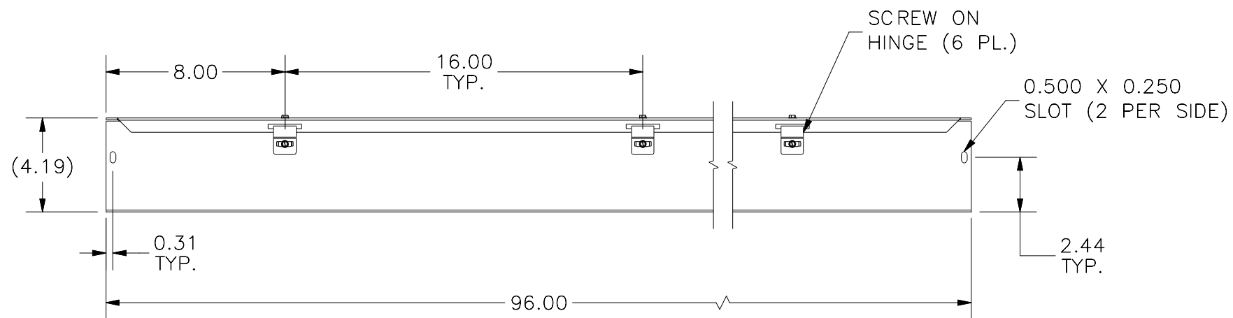
FRONT VIEW
