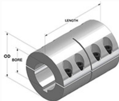
Two-Piece Industry Standard Clamping Coupling with Keyway
