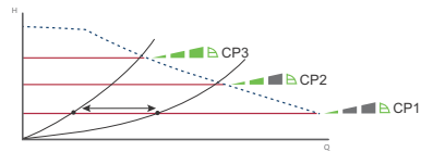
Fig. 18 Three constant-pressure curves/settings
