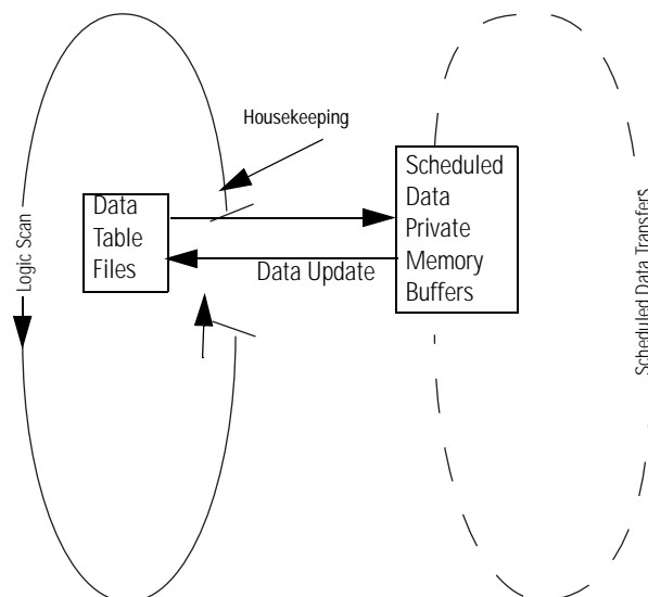
SLC 500 Program Scan Data Tables Files Housekeeping 1747-SCNR Scheduled Data
