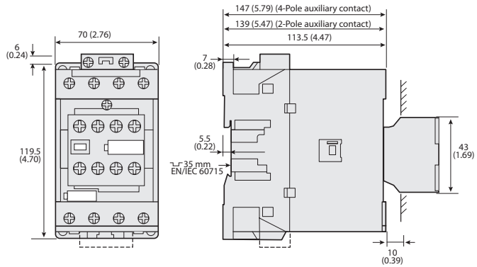
Figure 61 - 100-E40...100-E52 4-Pole Contactors with Front-mounted Auxiliary Contact
