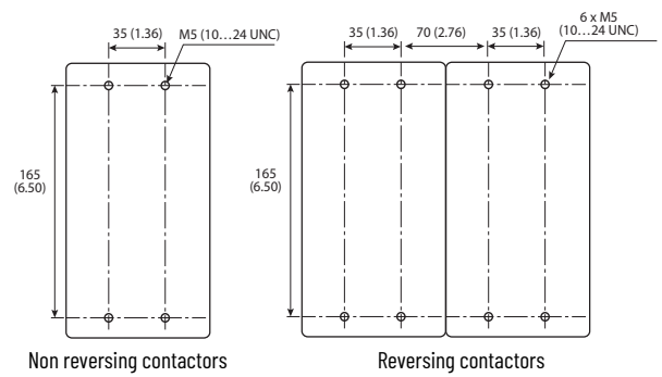
Figure 82 - 100-E265...100-E370 Contactors
