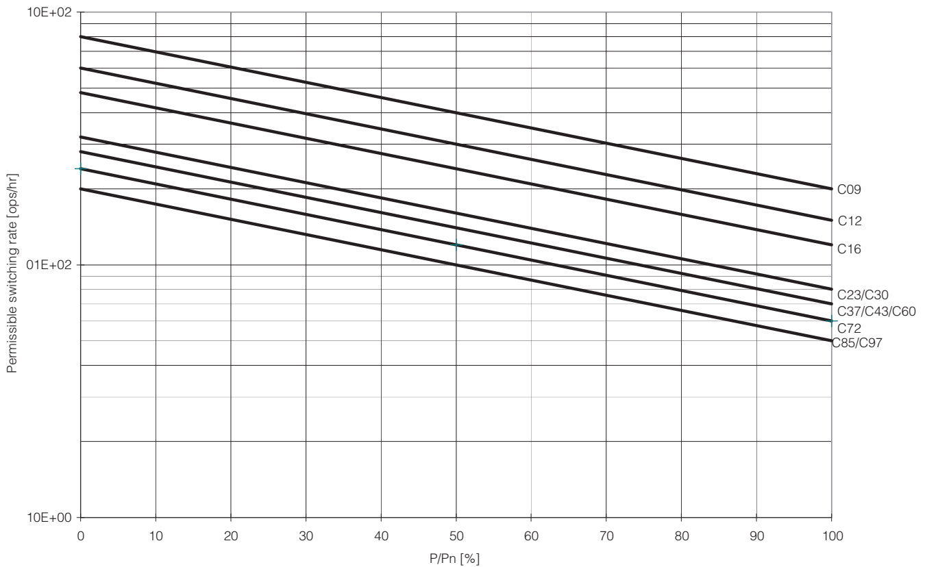
Figure 22 - AC-4, Inching of squirrel-cage motors; U_e = 230...460V , Starting time t_A = 0.25\text{ s}
