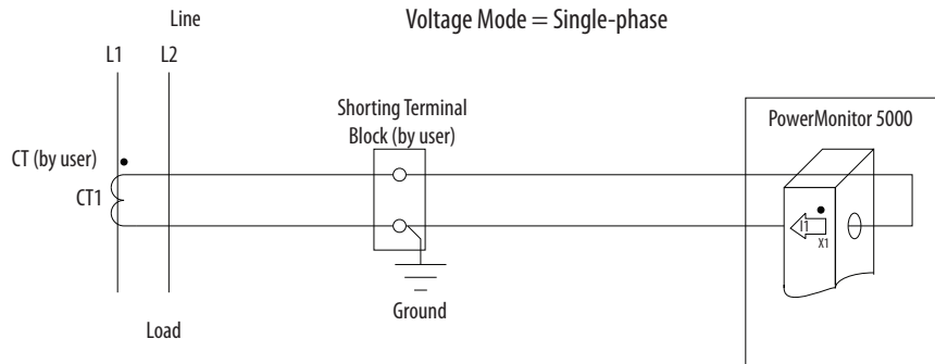
Figure 19 - Diagram I4 - Single Phase, 1 CT
