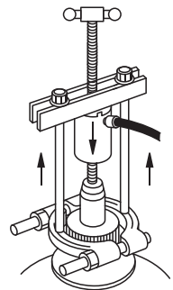
Bearing Puller shown with Crosshead Puller attachment. ▶
