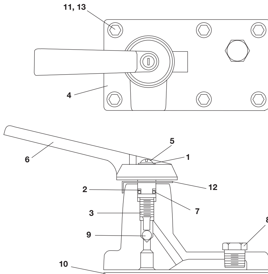
Figure 1, VM-2 Manual Valve
