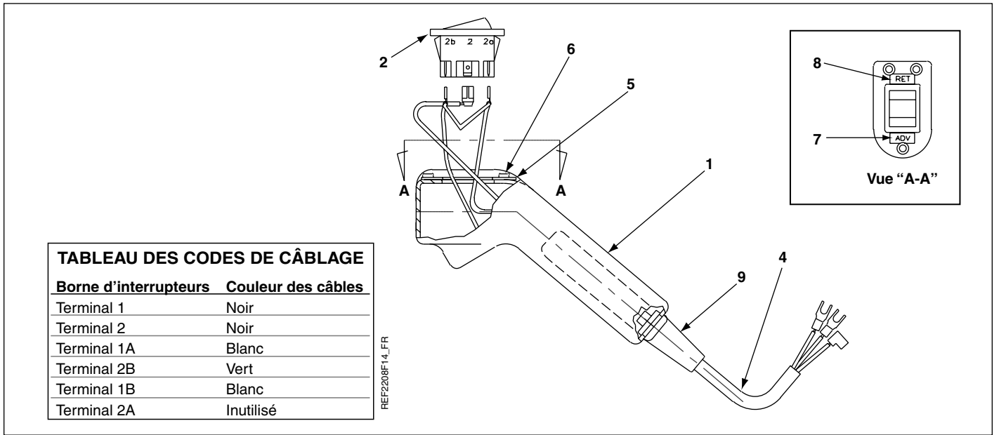
Figure 15, Pupitre mobile
