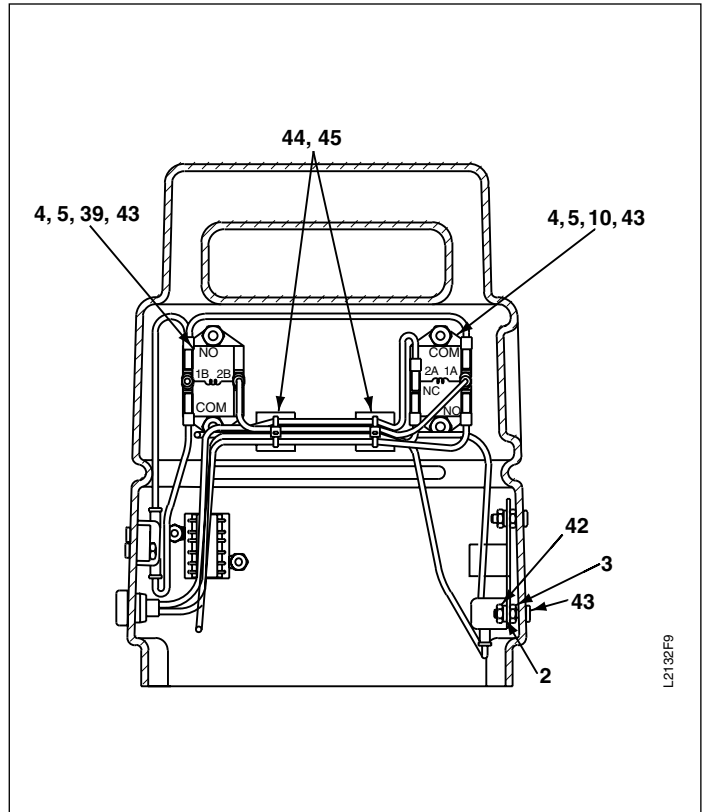
Figure 11, Shroud Wiring - Front of Motor
