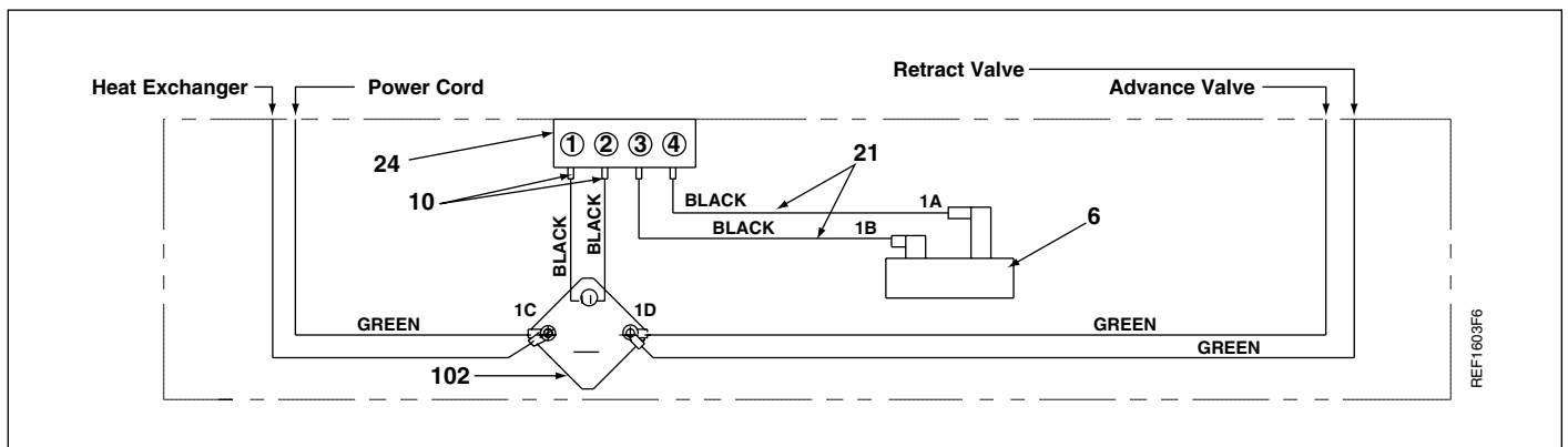
Figure 9, Wiring Diagram
