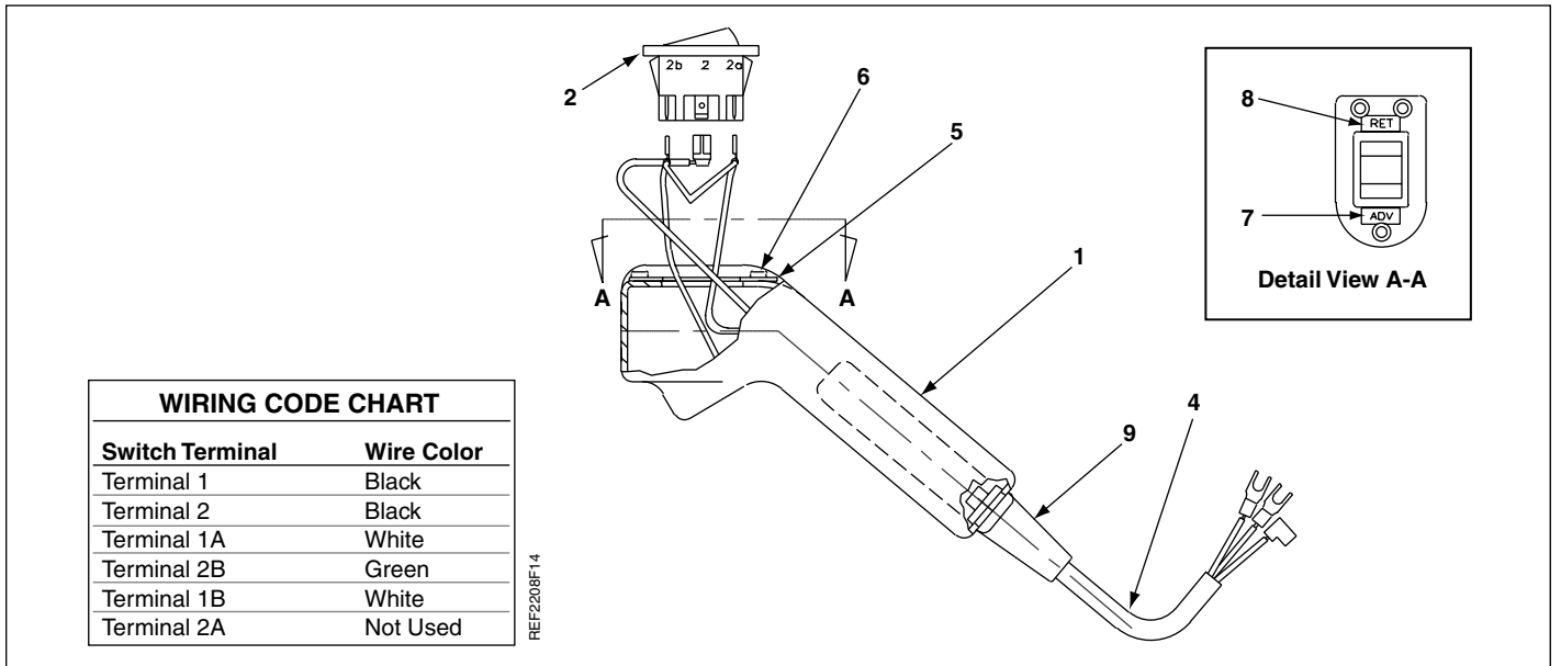
Figure 15, Pendant Assembly
