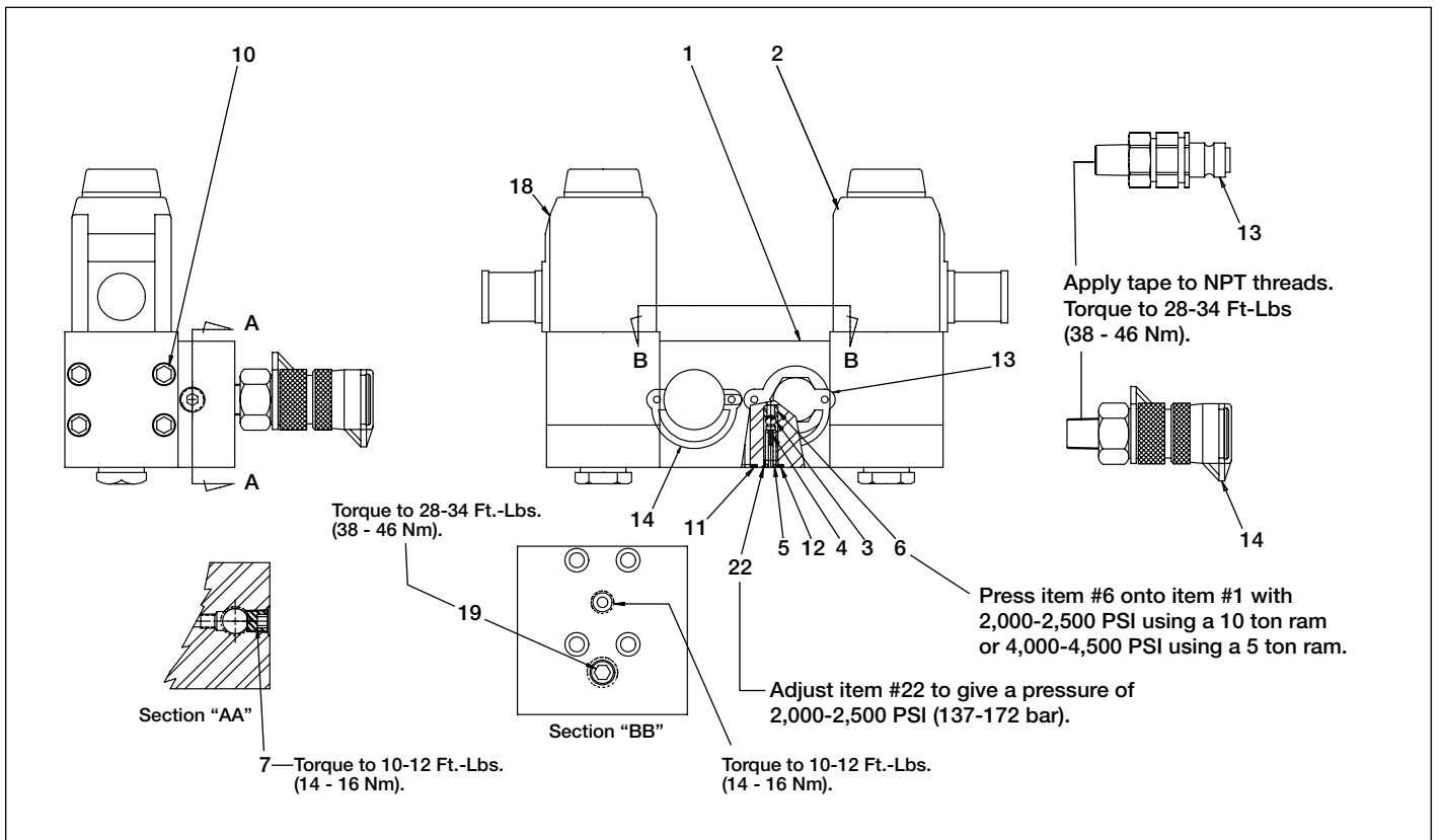
Figure 16, Poppet Valve
