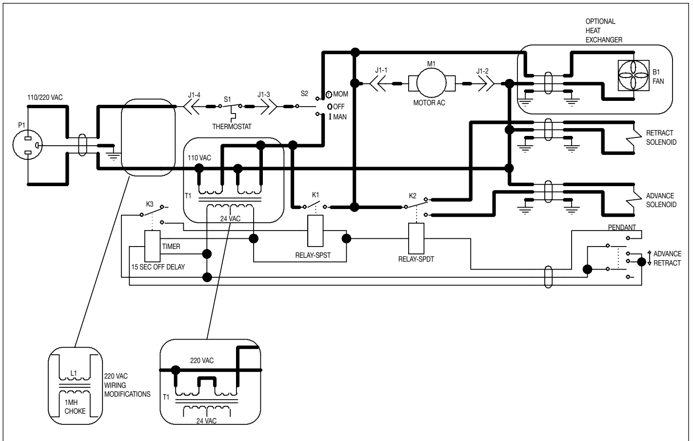
Figure 20, Electrical Schematic
