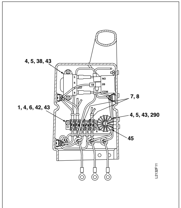
Figure 13, Shroud Wiring - Right of Motor
