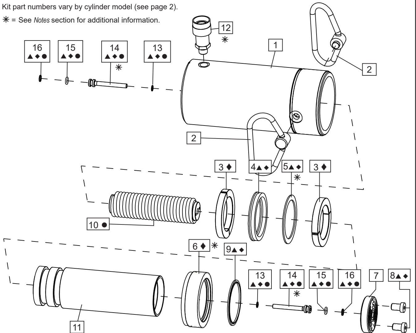
Fig. 1, Cylinder Assembly
