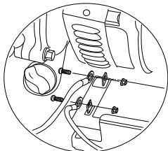
Figure 4-5. Battery Connection
