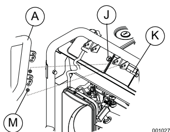
Figure 2-10. Handle Assembly
