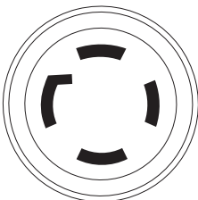
Figure 2-6. Prise 120/240 VCA, 30 A NEMA 14-30R
