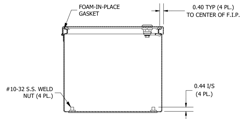
SECTION A-A (INSIDE TOP OF ENCL.)
