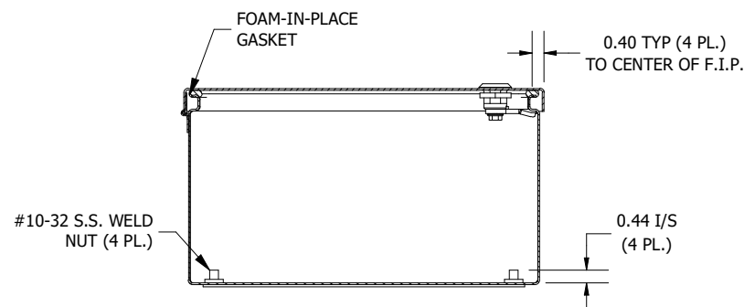
SECTION A-A (INSIDE TOP OF ENCL.)
