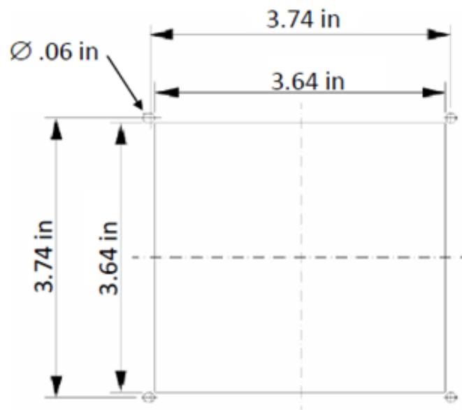
Mounting Cutout
