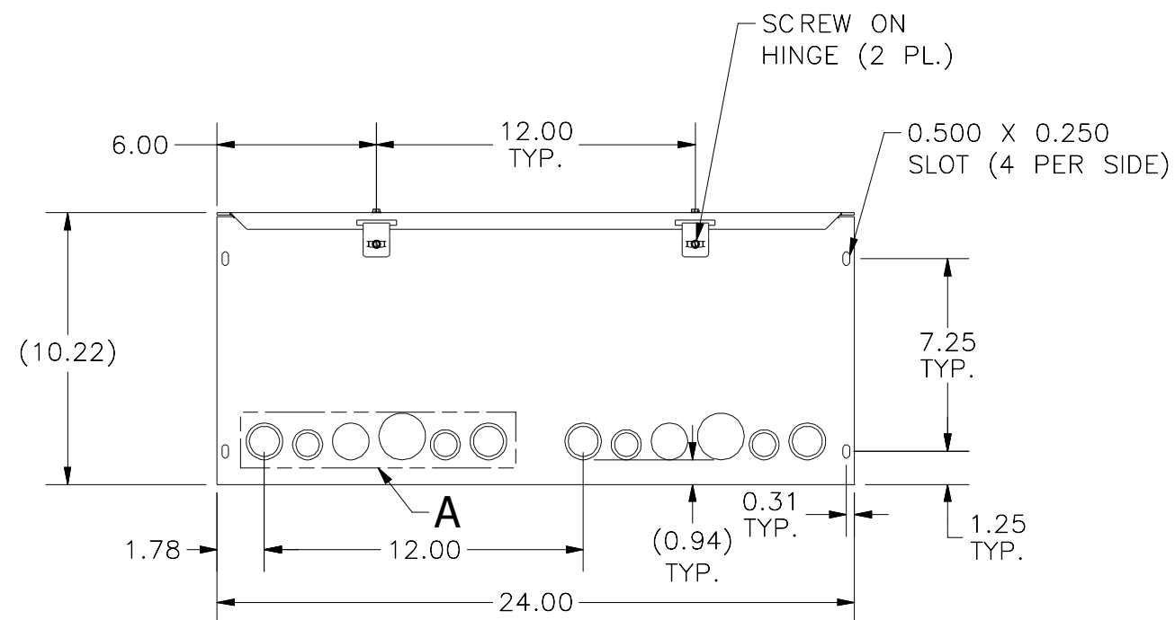
FRONT VIEW
