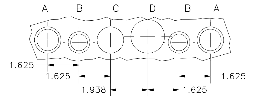
DETAIL A (2 PL. PER SIDE) PATTERN DESCRIPTION
