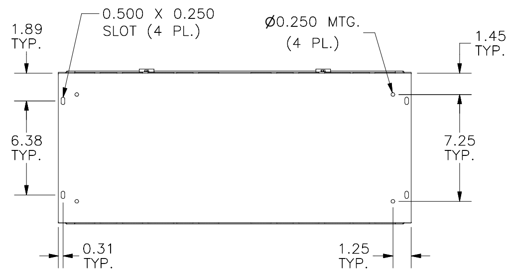
BOTTOM VIEW
