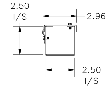
RIGHT VIEW
