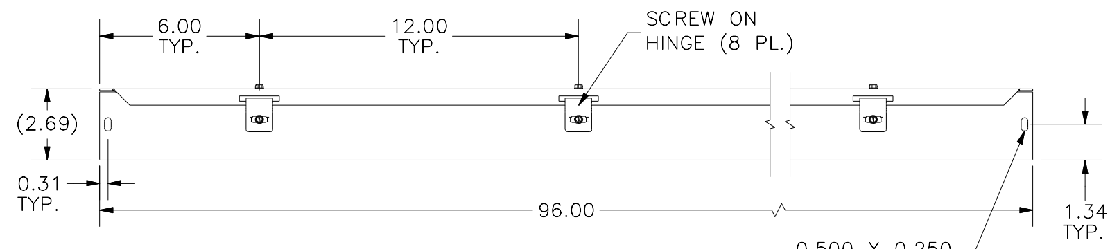
FRONT VIEW
