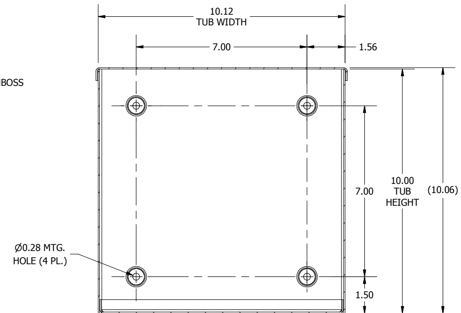
SECTION B-B (INSIDE BACK OF ENCL.)
