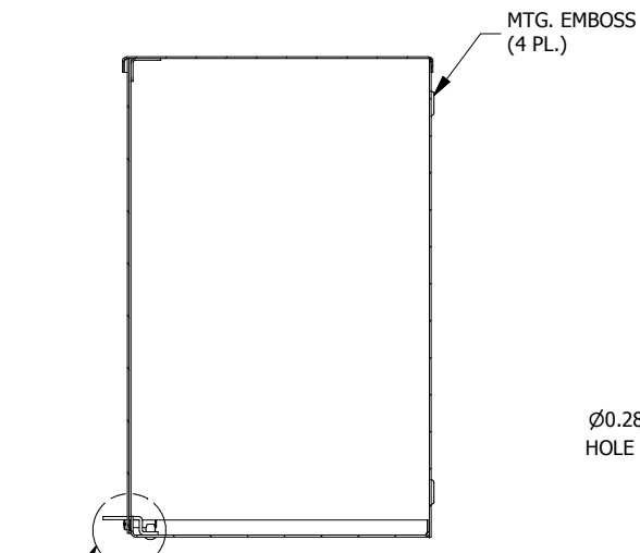
SECTION A-A (INSIDE LEFT OF ENCL.)
