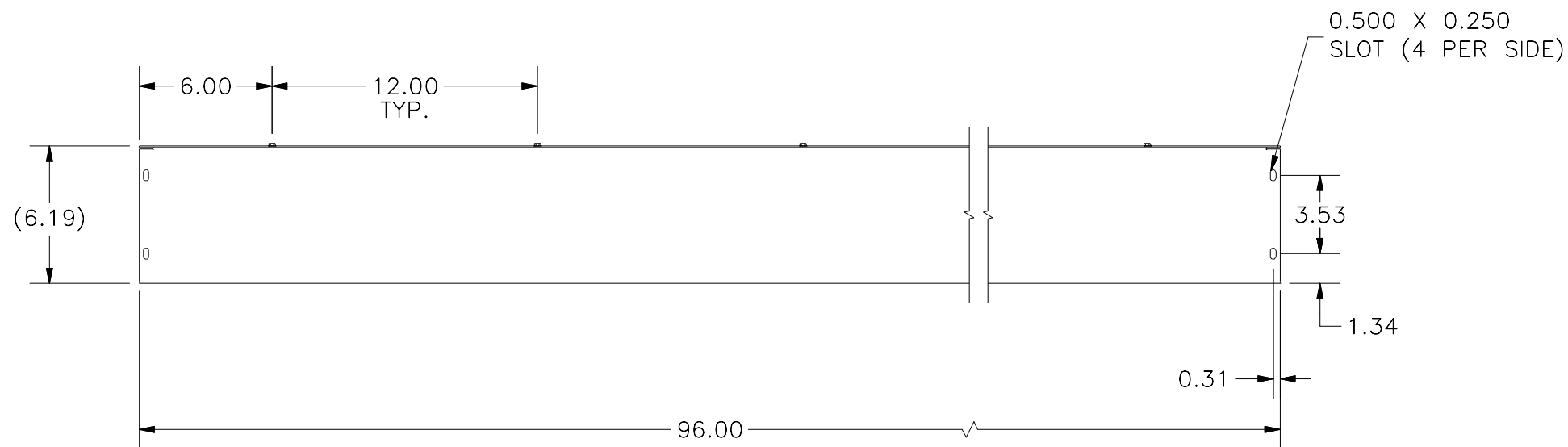
FRONT VIEW
