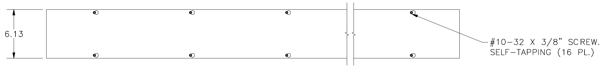
TOP VIEW
