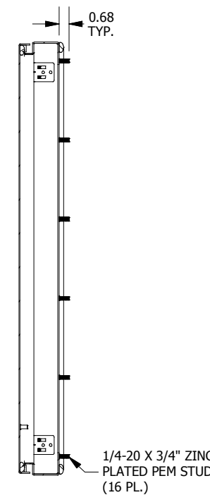
SECTION A-A (INSIDE LEFT OF ENCL.)
