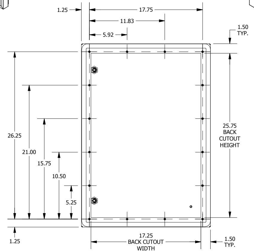
BACK VIEW
