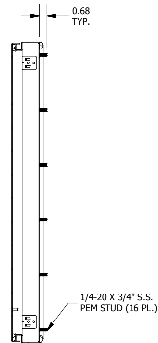
SECTION A-A (INSIDE LEFT OF ENCL.)
