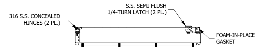
SECTION B-B (INSIDE TOP OF ENCL.)
