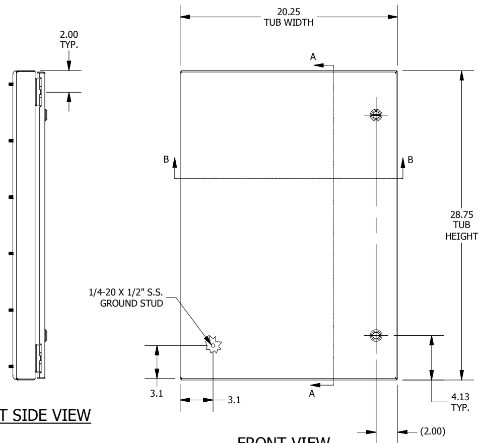
FRONT VIEW
