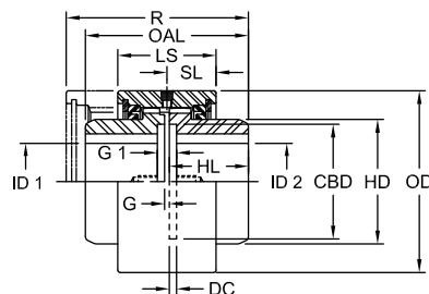
CFR Type Flex-Rigid Coupling
