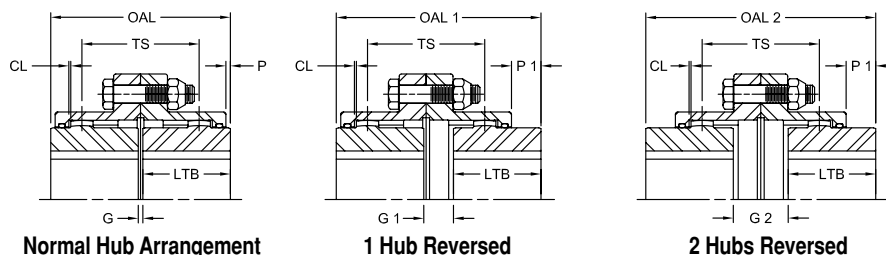
Normal Hub Arrangement
