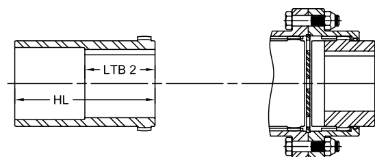
Alternate Type hub shaft contact is deep inside hub
