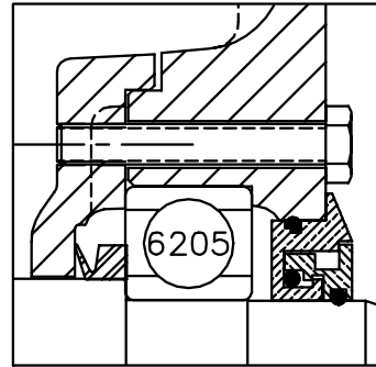
PULLEY END DETAIL
