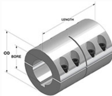
Metric Two-Piece Industry Standard Clamping Coupling with Keyway
