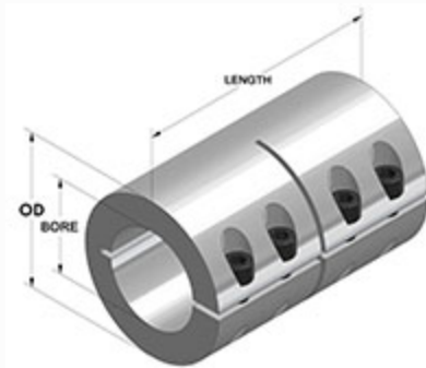
Metric One-Piece Industry Standard Clamping Coupling
