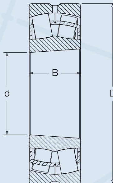
TAPERED BORE
