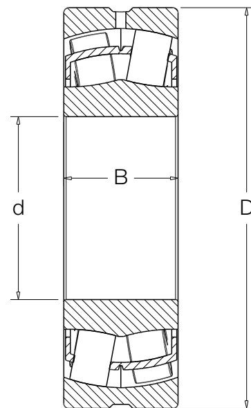
STRAIGHT BORE
