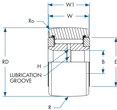
CAM YOKE ROLLER CROWNED (CCYR)
