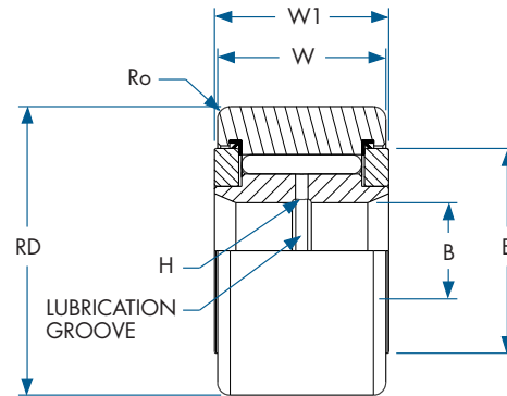
CAM YOKE ROLLER CYLINDRICAL (CYR)
