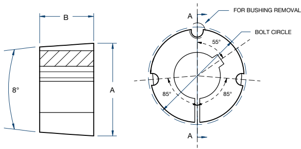
No. 1008-3030 Bushings
