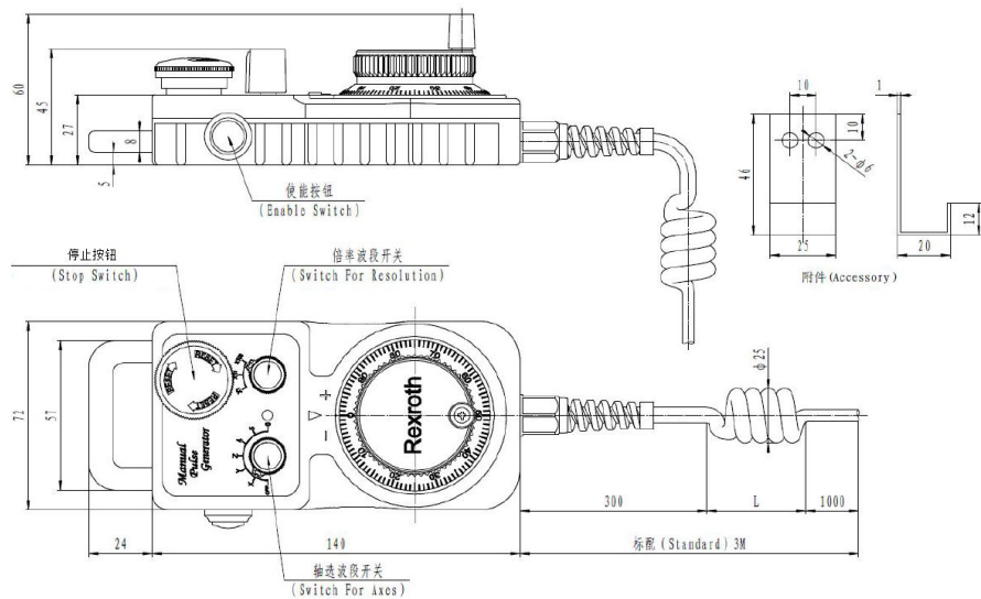
Fig. 11-2: Dimensions
