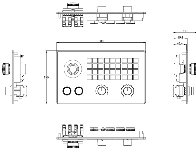
Fig. 5-10: VAM82.1-USB-NF-TA-TA-VE-MA-NNNN dimensions
