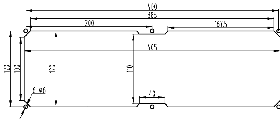
Fig. 5-15: Cut out of VAM81.1-USB-NF-TA-TA-VE-MA-NNNN
