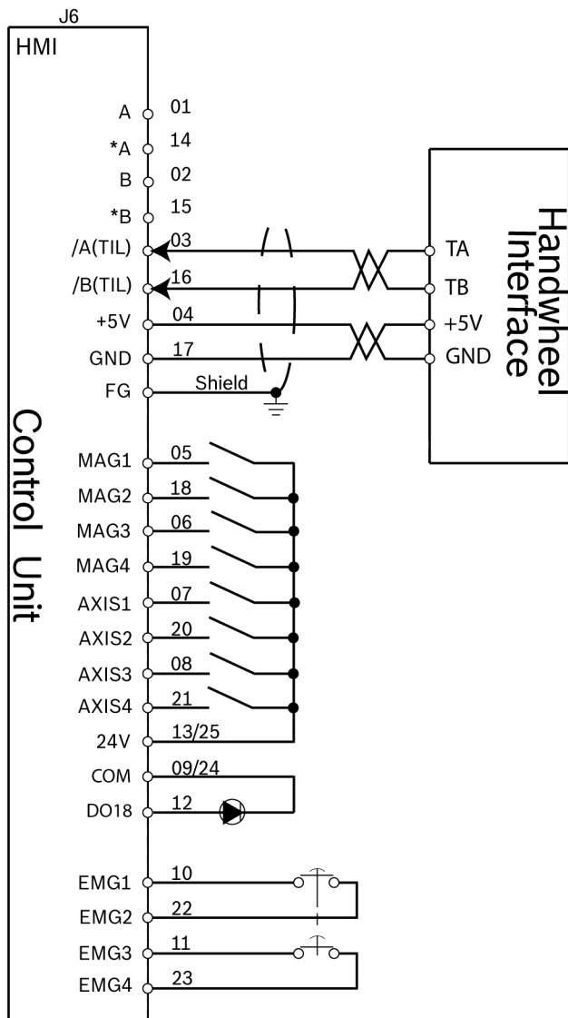
Fig. 9-6: Handwheel unit - Output of type open collector
