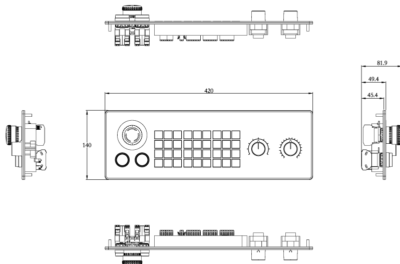
Fig. 5-8: VAM81.1-USB-NF-TA-TA-VE-MA-NNNN dimensions
