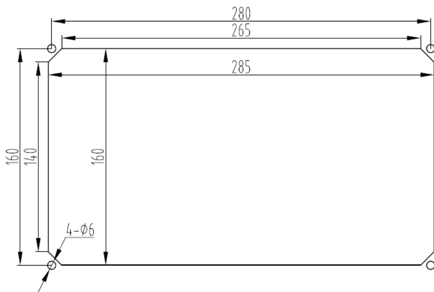
Fig. 5-16: Cut out of VAM82.1-USB-NF-TA-TA-VE-MA-NNNN
