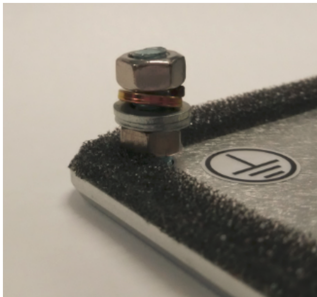
Fig. 5-18: Recommend GND terminal with nuts
