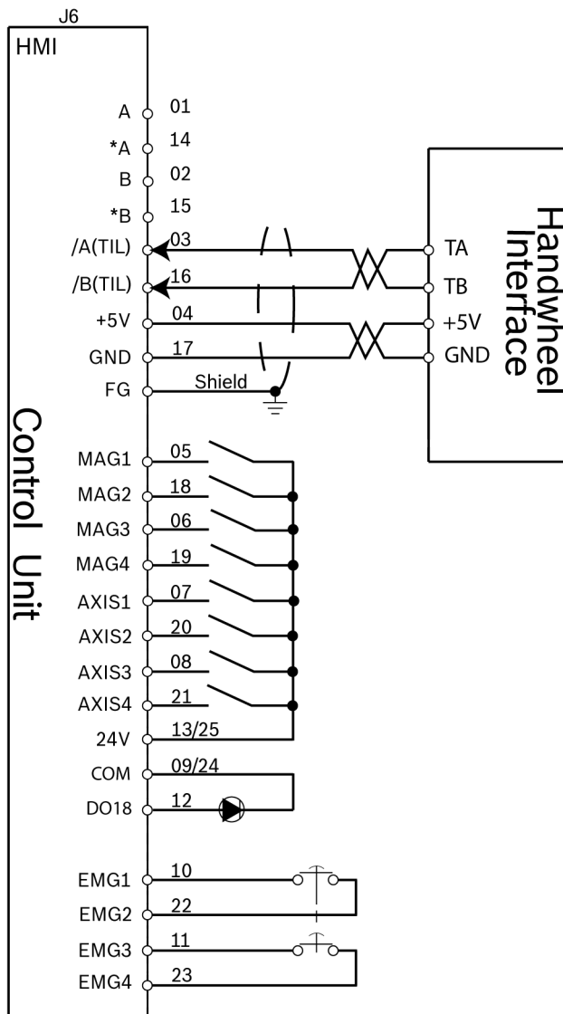
Fig. 8-6: Handwheel unit - Output of type open collector
