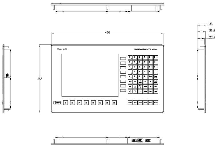
Fig. 5-6: VDP81.1FKN-C1-NN-EN dimensions
