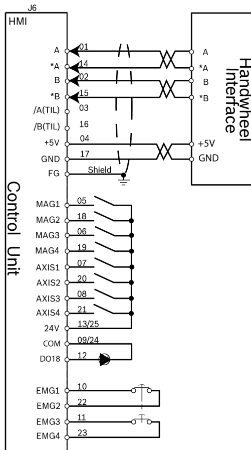
Fig. 9-7: Handwheel unit - Input of type differential
