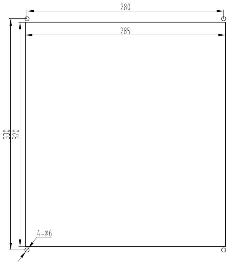
Fig. 5-14: Cut out of VDP82.1FKN-C1-NN-EN
