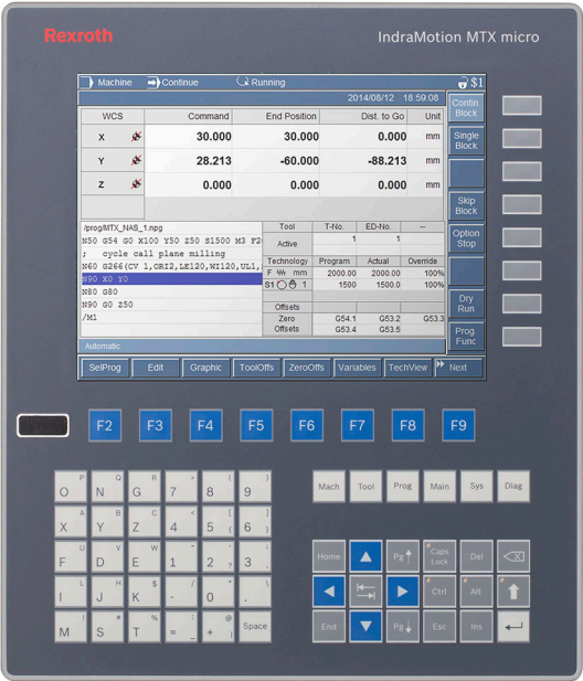
Fig. 5-2: Front panel of the VDP82.1FKN-C1-NN-EN
