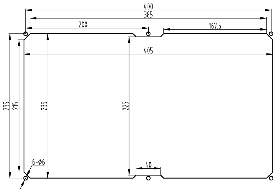
Fig. 5-13: Cut out of VDP81.1FKN-C1-NN-EN
