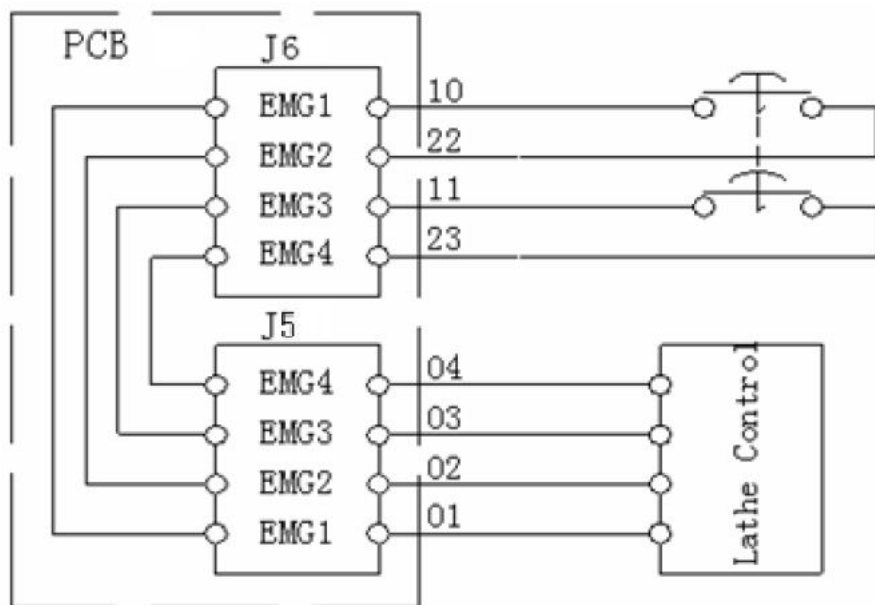
Fig. 9-8: Stop Switch in handwheel unit signal connection
