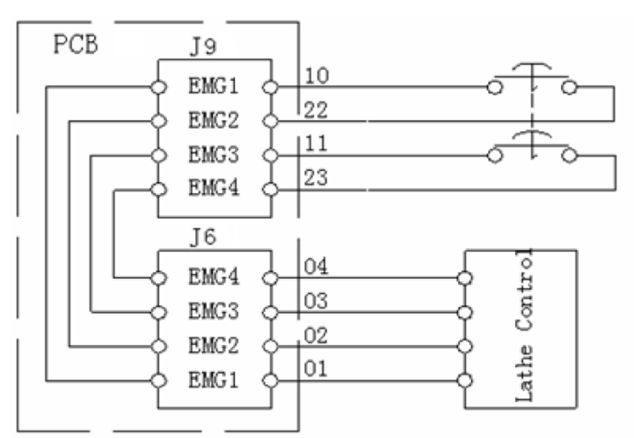
Fig. 8-8: Stop Switch in handwheel unit signal connection
