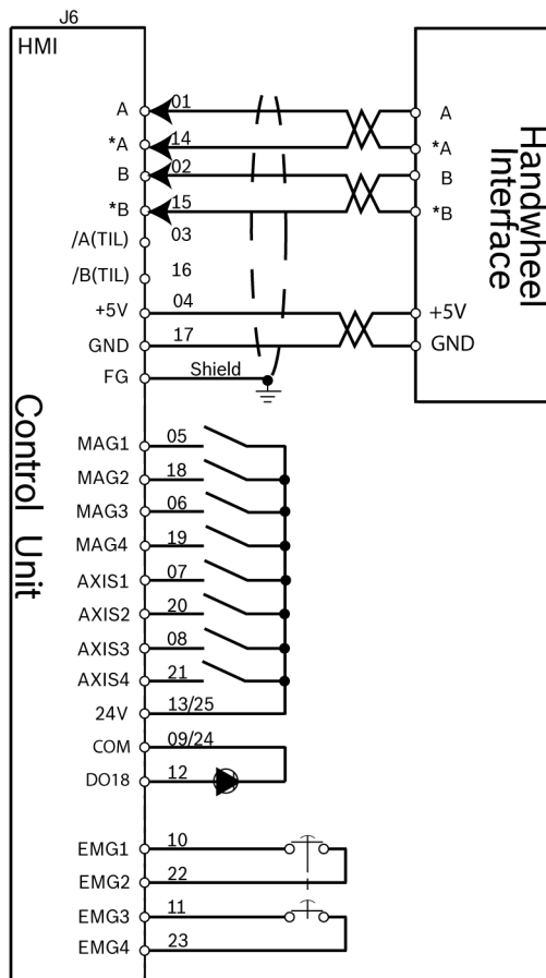
Fig. 8-7: Handwheel unit - Input of type differential
