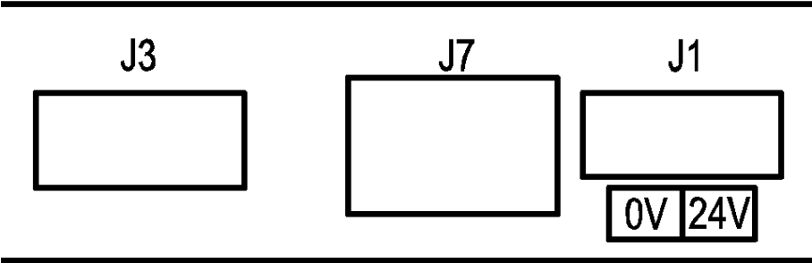
Fig. 6-3: Interface view of VDP81.1 and VDP82.1 HMI operator panel
