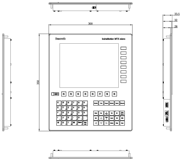
Fig. 5-7: VDP82.1FKN-C1-NN-EN dimensions
