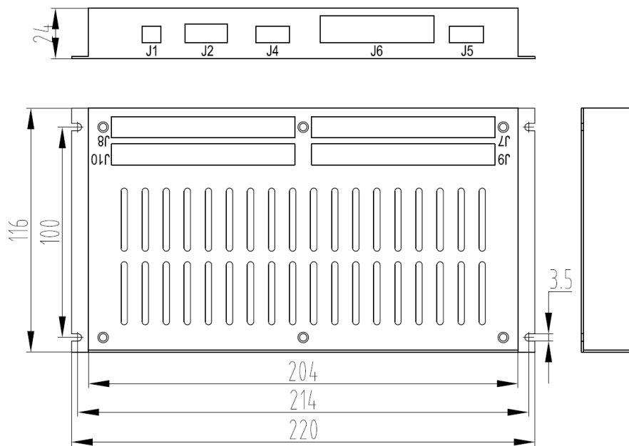
Fig. 5-12: VAC06.1S-MU1-NNNN dimensions
