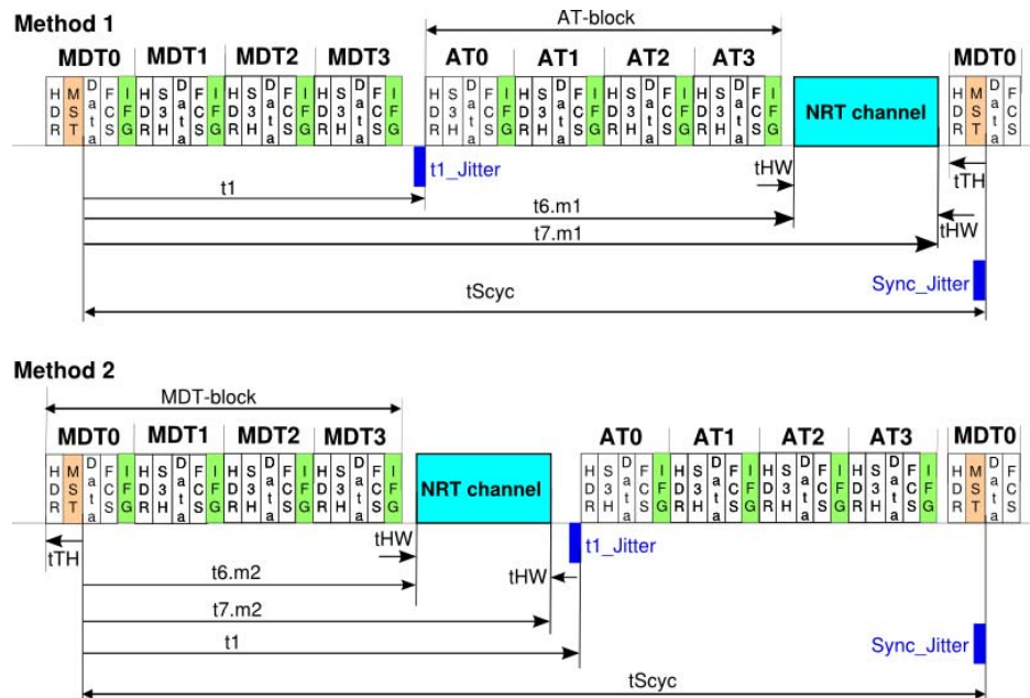
Fig. 8-2 Calculation of t_6 and t_7n
