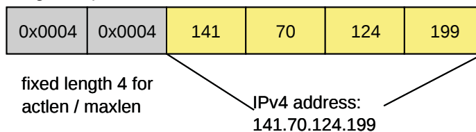
Fig. 8-4 Structure of IP address S-0-1020
