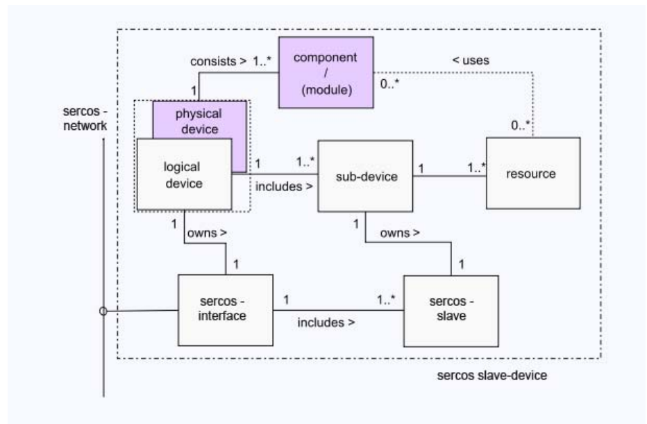
Fig. 2-5 Structure diagram of a sercos slave with physical sequence
