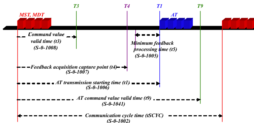
Fig.6-2 Timing of the communication layer
