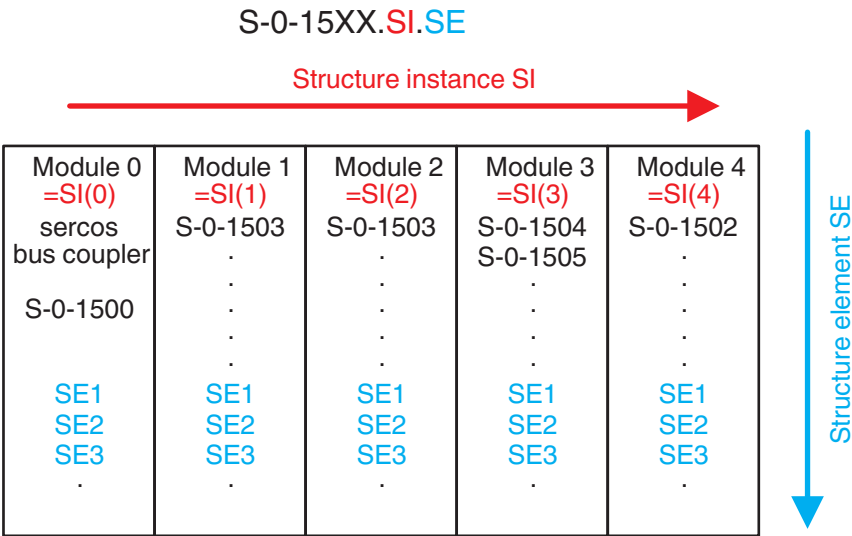
Fig. 2-8 Modular I/O station
