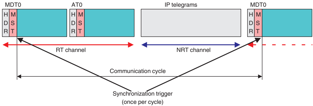
Fig. 3-3 Synchronization via MDT0.
