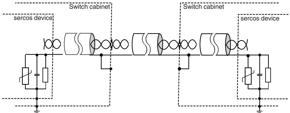
Fig. 4-11 First example of a parallel RC shield grounding version
