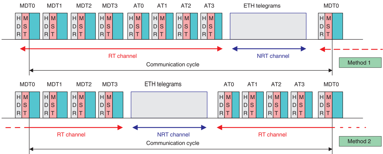
Fig. 3-2 Two methods for configuring a communication cycle
