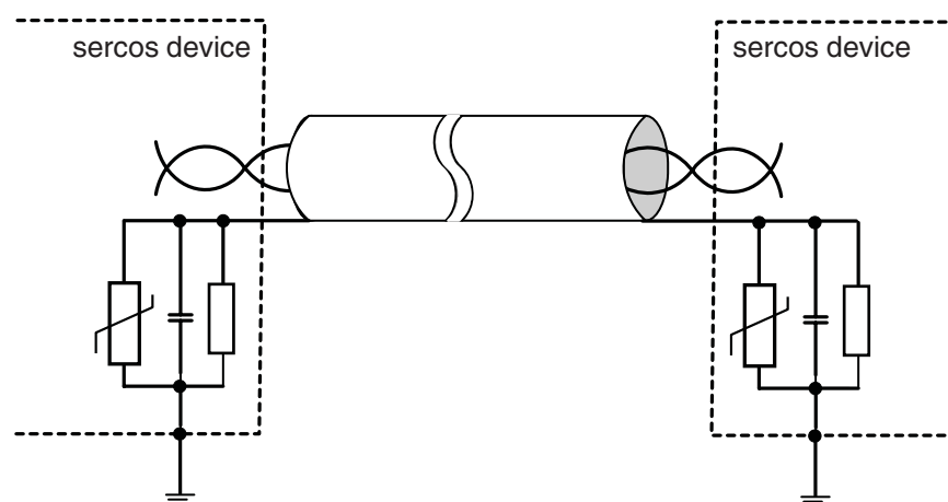
Fig. 4-10 Parallel RC shield grounding
