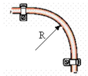
Fig. 4-5 Observe the minimum bending radius
