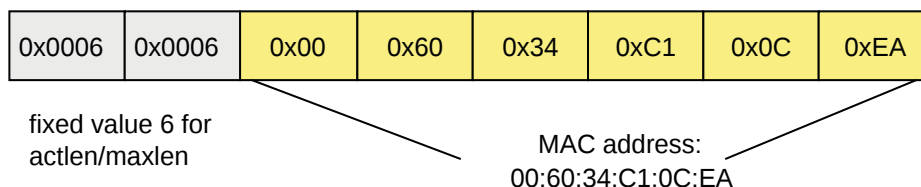
Fig. 8-3 MAC address S-0-1019
