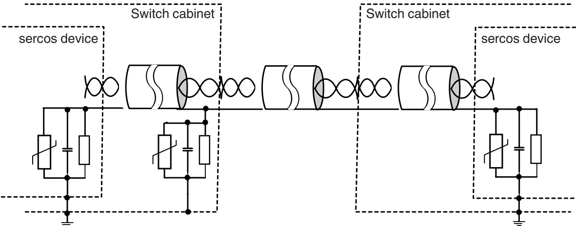
Fig. 4-14 Fourth example of a parallel RC shield grounding version
