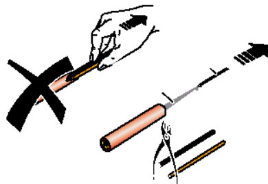
Fig. 4-6 Do not pull at the individual wires
