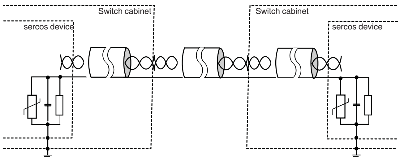
Fig. 4-13 Third example of a parallel RC shield grounding version
