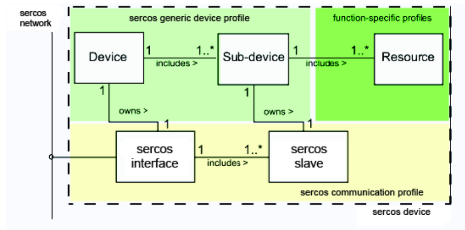
Fig. 2-10 Structure diagram of a sercos slave device
