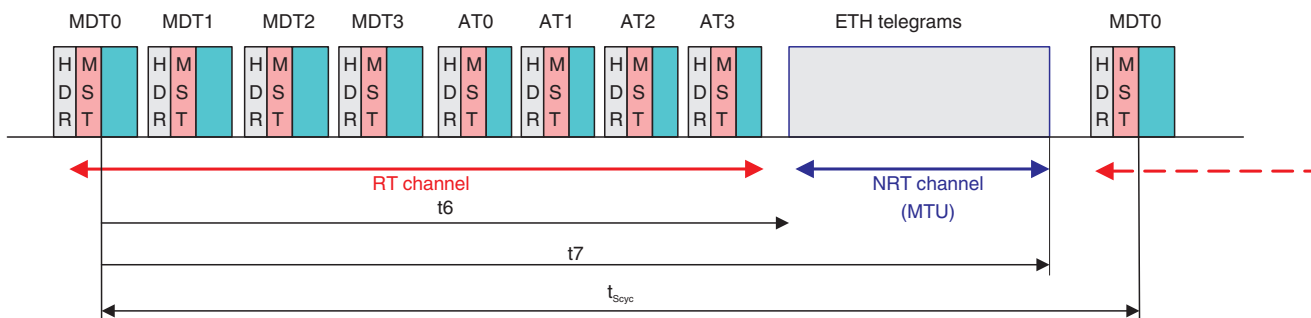
Fig. 3-5 Time parameters of the NRT channel
