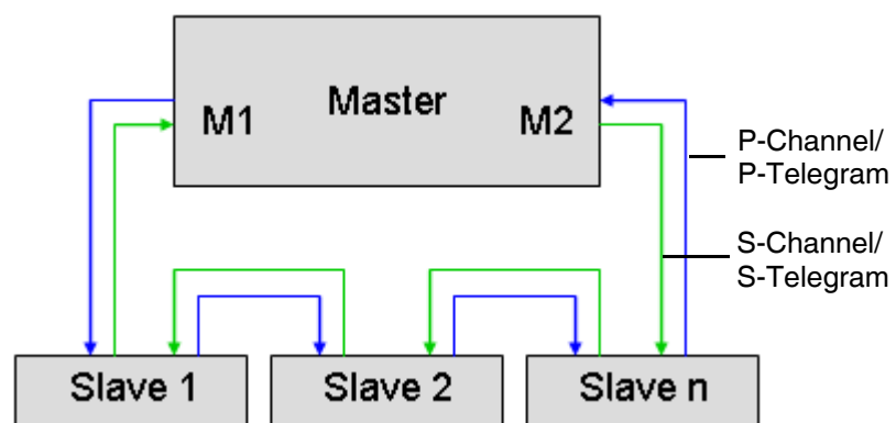
Fig. 2-1 Ring structure (double ring)
