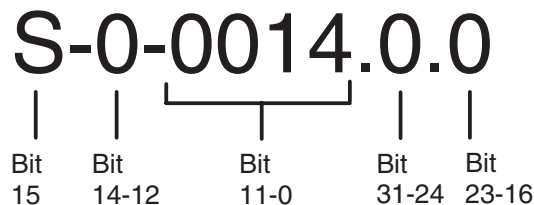
Fig. 8-1 IDN structure
