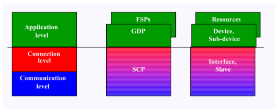
Fig. 2-3 Communication model for the various layers
