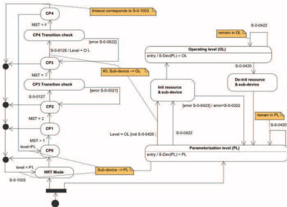
Fig. 5-1 sercos communication state machine
