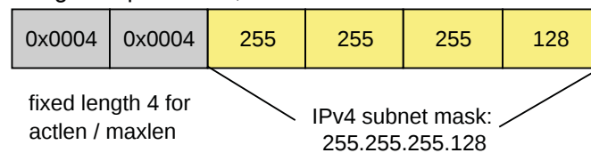
Fig. 8-5 Structure of the subnet mask S-0-1021
