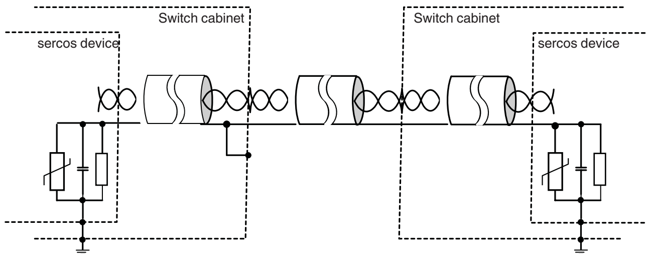
Fig. 4-12 Second example of a parallel RC shield grounding version
