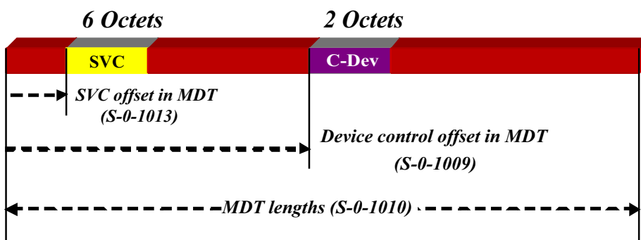
Fig.6-3 Telegram structure of the communication layer
