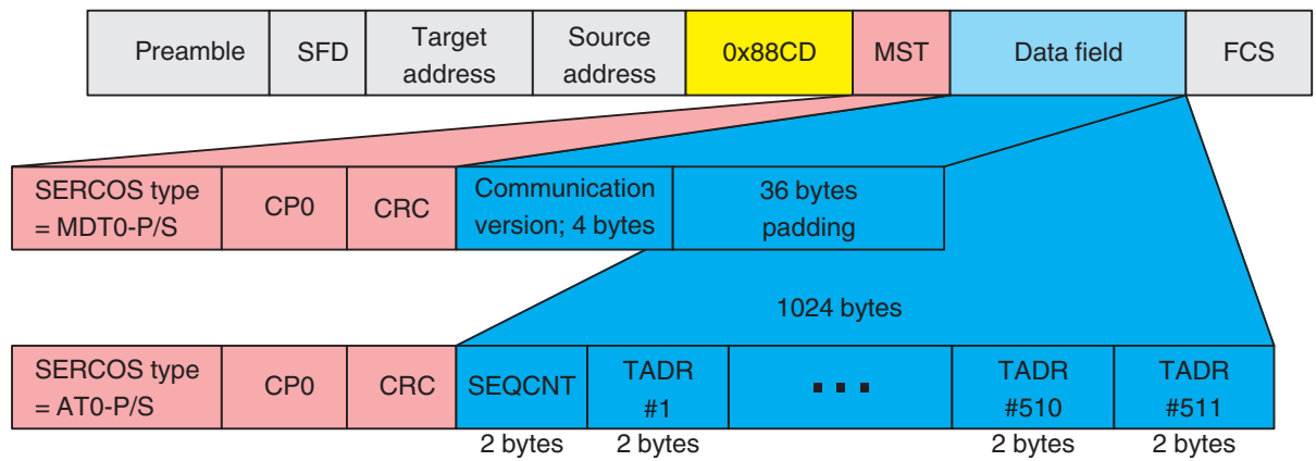
Fig. 3-4 Structure of the MDT and AT array
