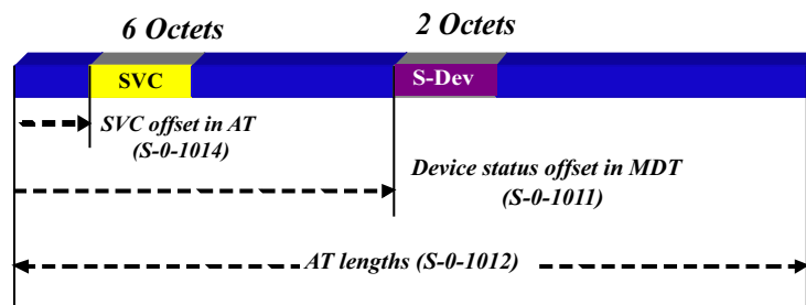
Fig. 2-4 Telegram structure of the communication layer
