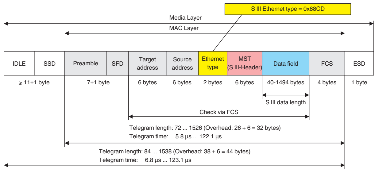
Fig. 3-1 General telegram structure for sercos MDT and AT telegrams
