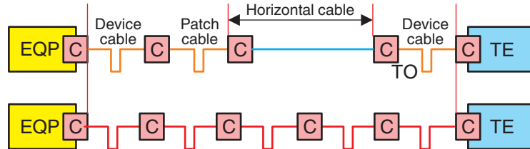
Fig. 4-1 Structure of the channel
