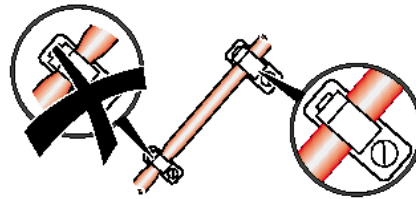
Fig. 4-7 Use cable clamps with large (wide) surface
