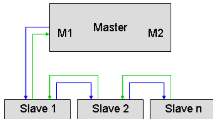
Fig. 2-2 Linear structure (single ring)
