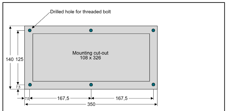
Fig.5-3: Mounting dimensions VAK 11.2
