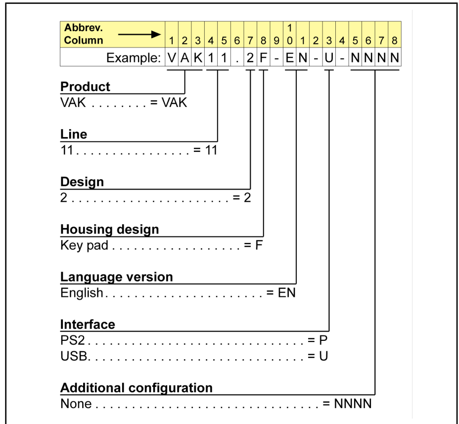
Fig.9-1: Type code designation VAK 11.2
