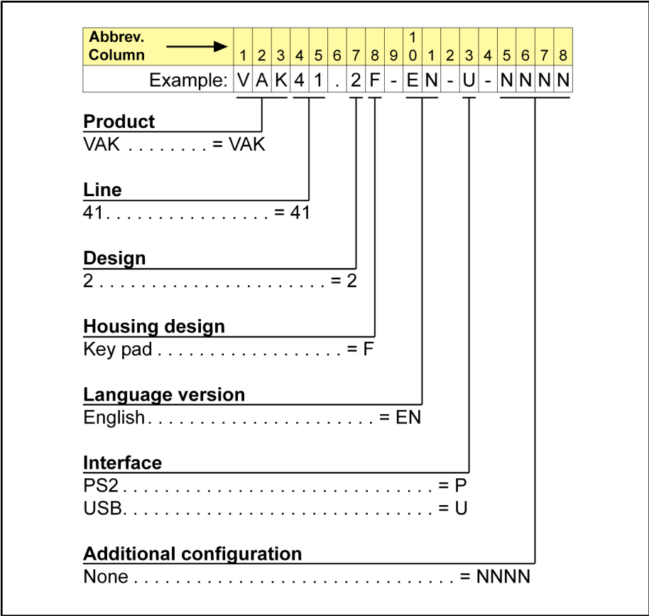
Fig.9-2: Type code designation VAK 41.2
