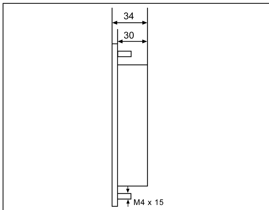
Fig.5-5: VAK 11.2 and VAK 41.2, side view
