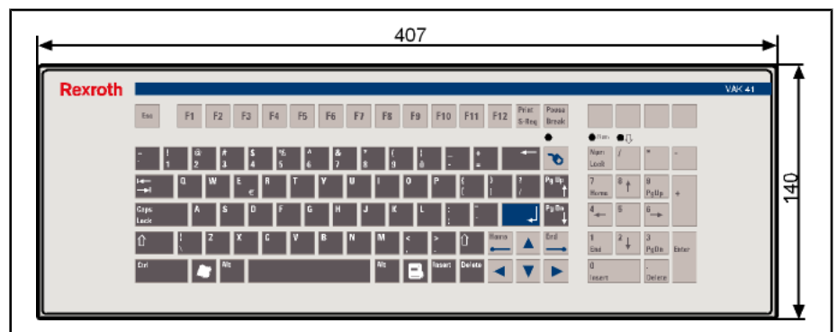
Fig.5-2: Housing dimensions VAK 41.2
