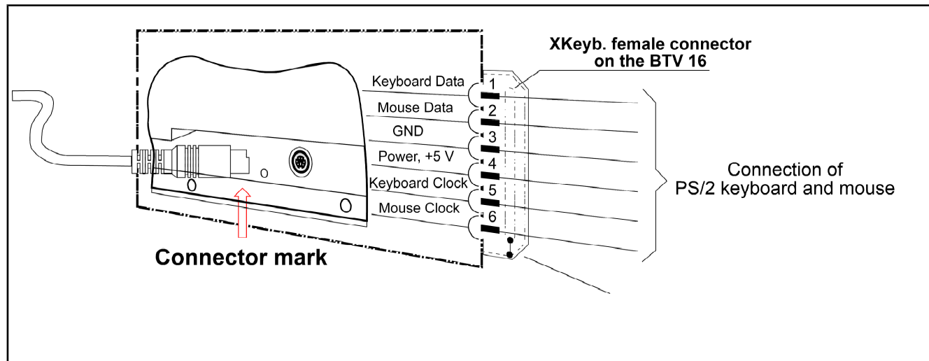
Fig.7-4: connection to an operator terminal BTV 16
