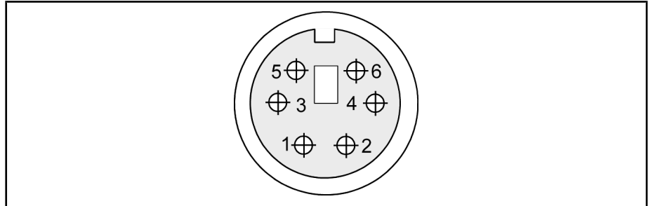
Fig. 7-1: Mini DIN PS/2 keyboard connector: View on the pins
