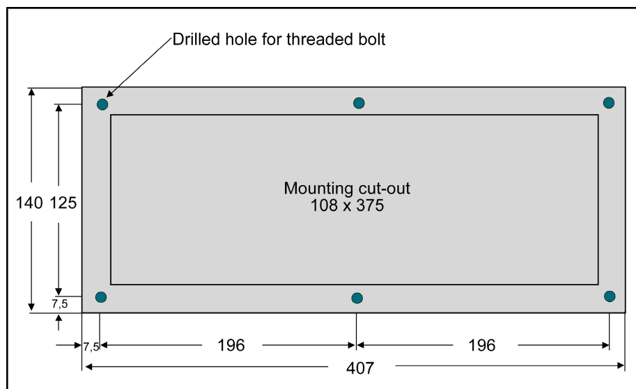
Fig.5-4: Mounting dimensions VAK 41.2
