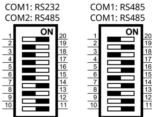
Fig. 16: Changeover switch position of COM1 and COM2 upon delivery
