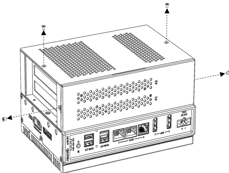
Fig. 7: Removing housing cover
