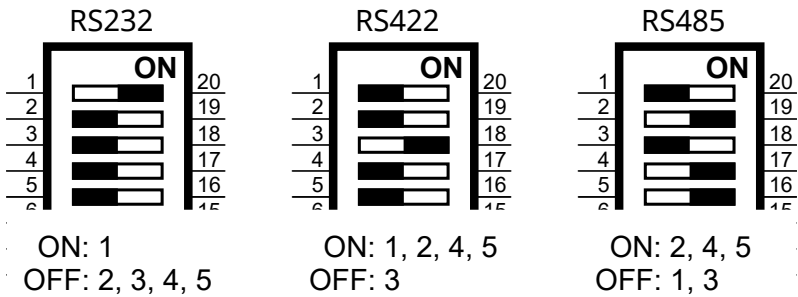
Fig. 14: Position of the changeover switches at COM1 for RS232, RS422 and RS485
