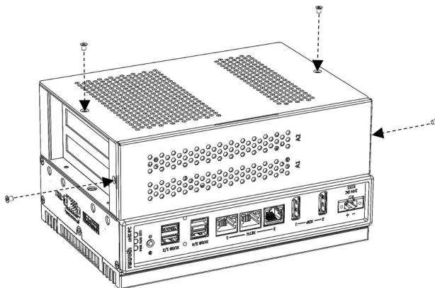
Fig. 10: Fastening the housing cover
