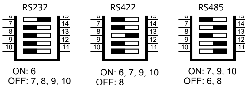
Fig. 15: Position of the changeover switches at COM2 for RS232, RS422 and RS485
