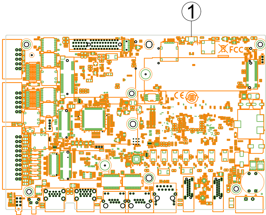
Fig. 20: Position of the battery plug Connection for battery
