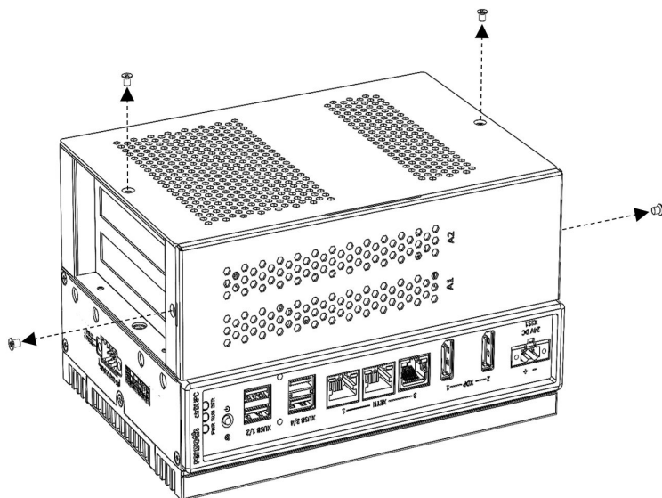
Fig. 18: Removing housing cover
