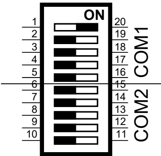
Fig. 13: Assigning the COM1 and COM2 changeover switches
