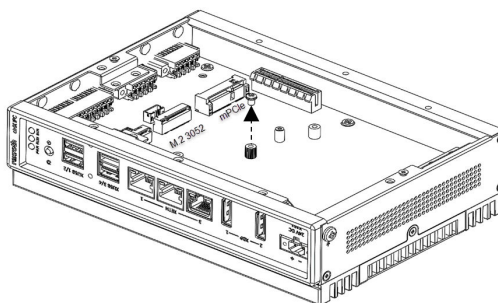
Fig. 11: Loosen the screw for the mPCIe module or the M.2 3052 module
