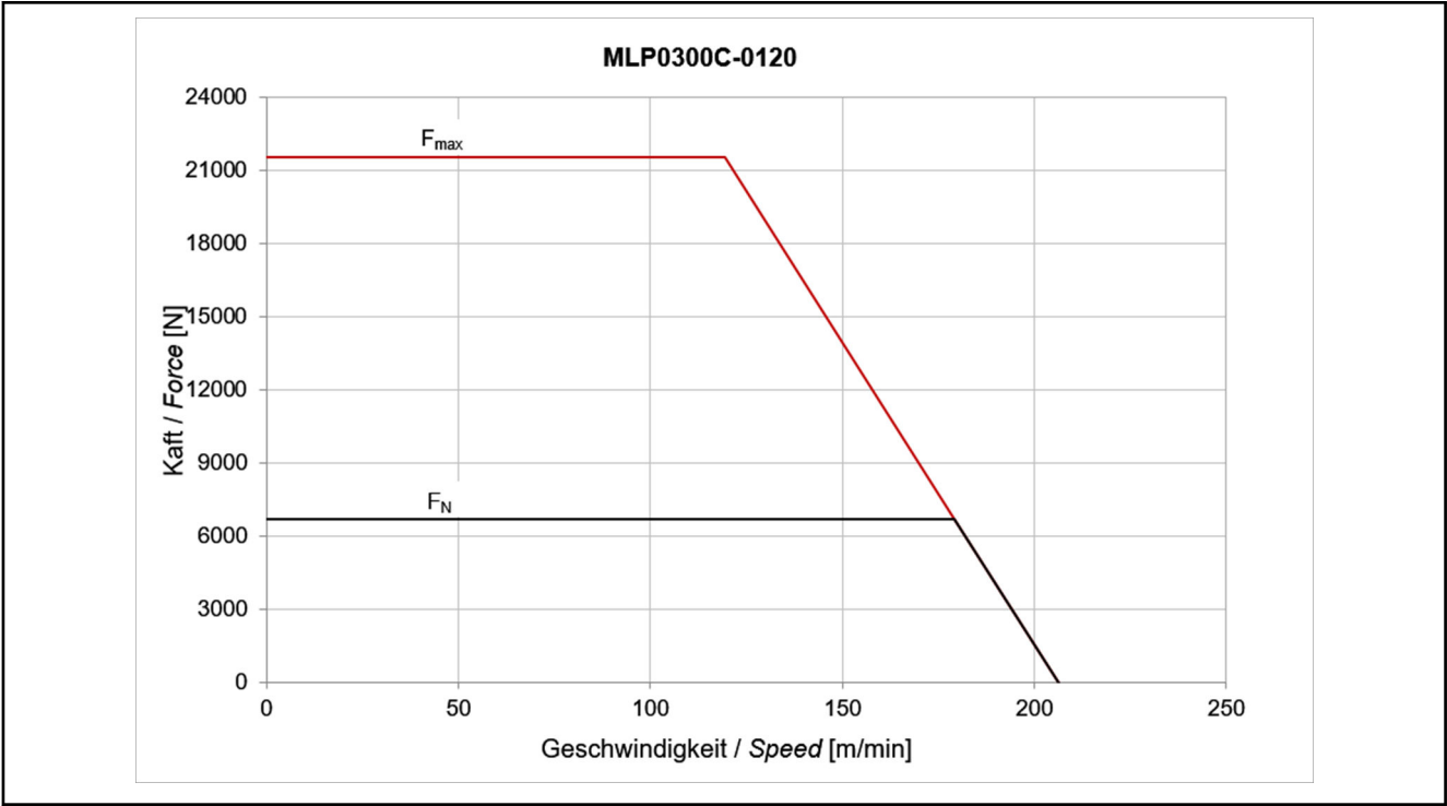
Fig. 4-72: Motor characteristic curves MLP300C-0120
