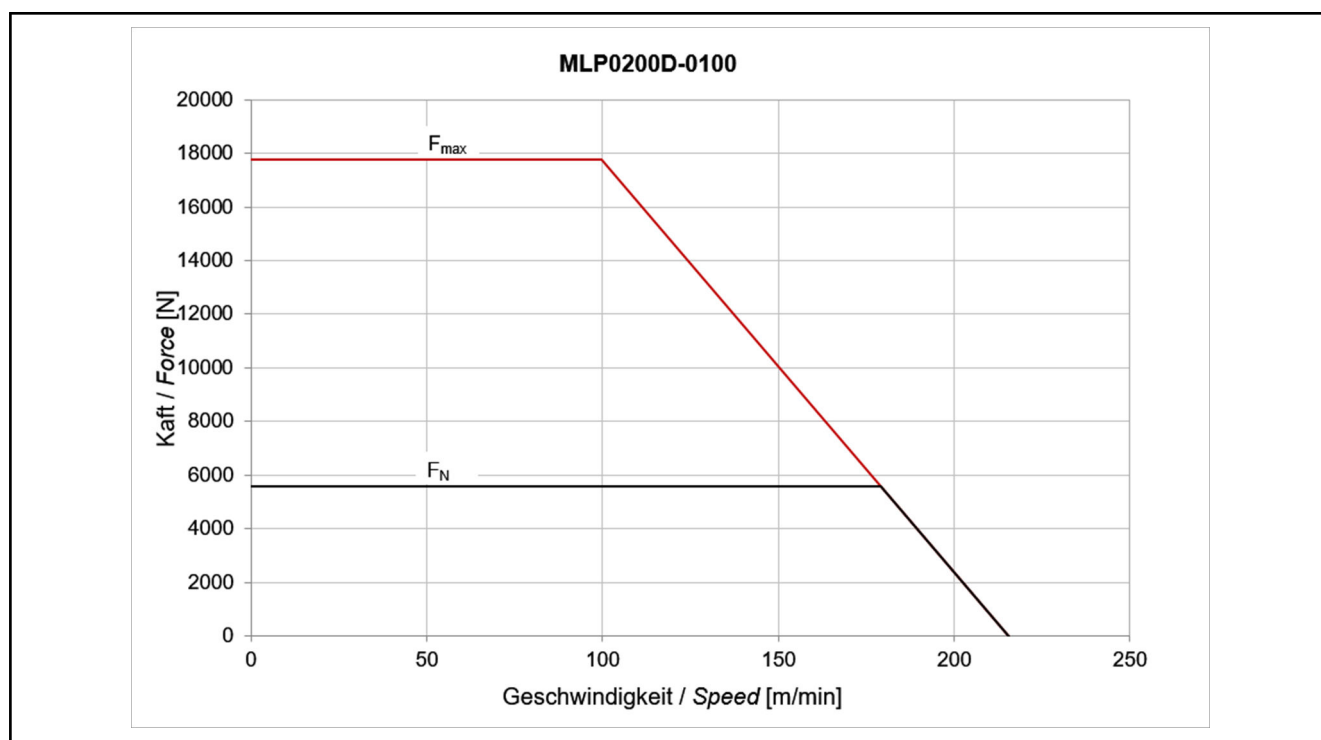
Fig. 4-60: Motor characteristic curves MLP200D-0100
