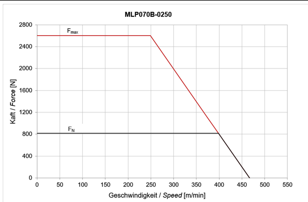
Fig. 4-16: Motor characteristic curves MLP070B-0250
