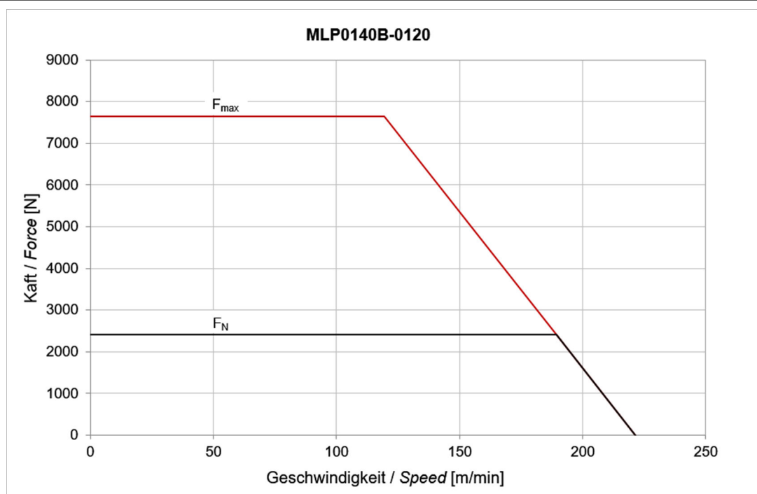
Fig. 4-42: Motor characteristic curves MLP140B-0120
