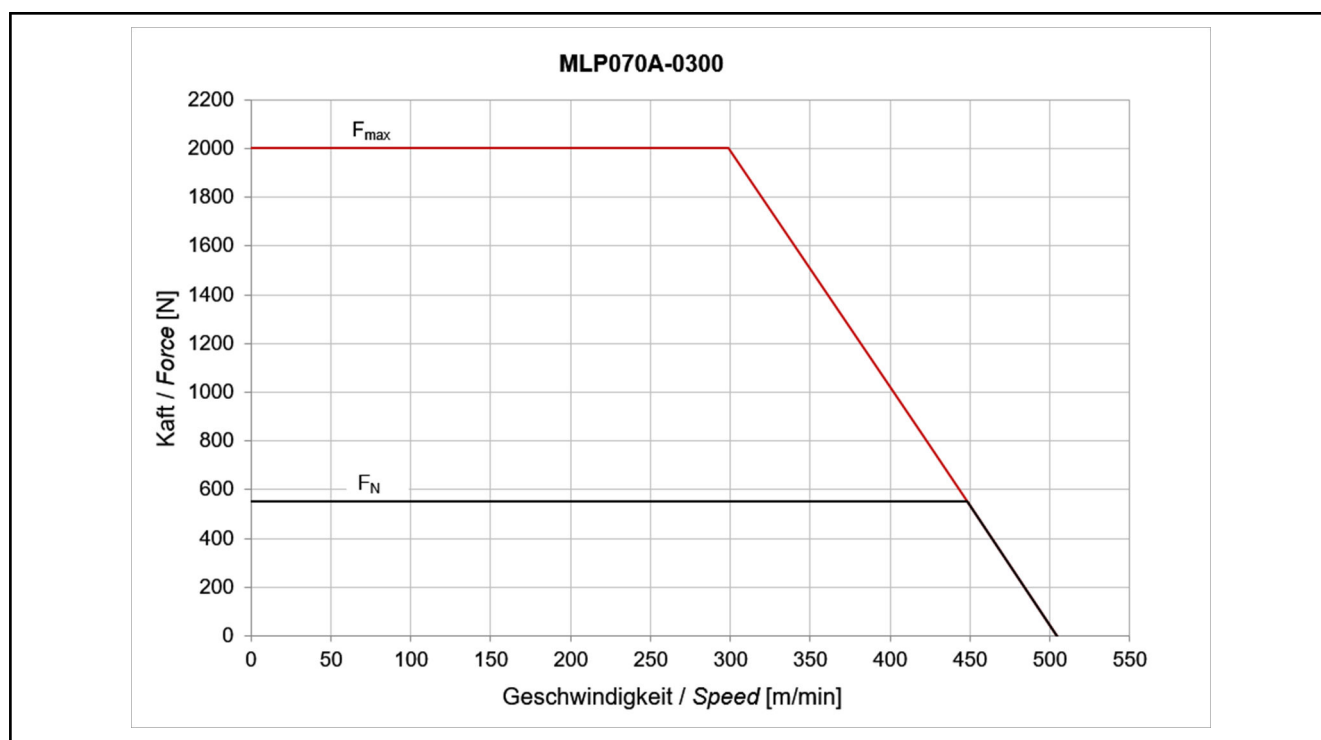
Fig. 4-12: Motor characteristic curves MLP070A-0300
