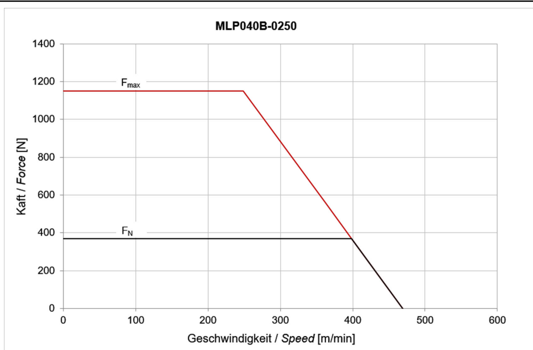
Fig. 4-6: Motor characteristic curve MLP040B-0250
