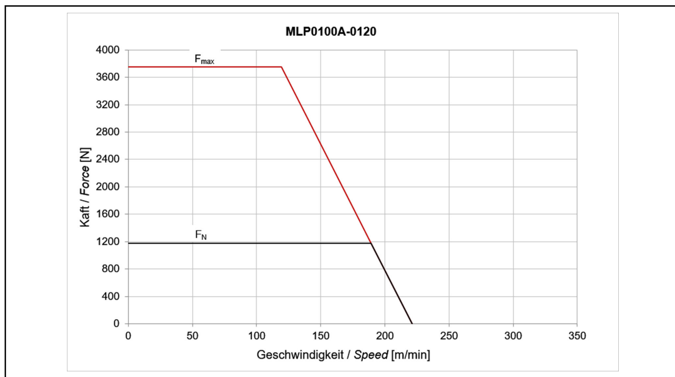
Fig. 4-24: Motor characteristic curves MLP100A-0120
