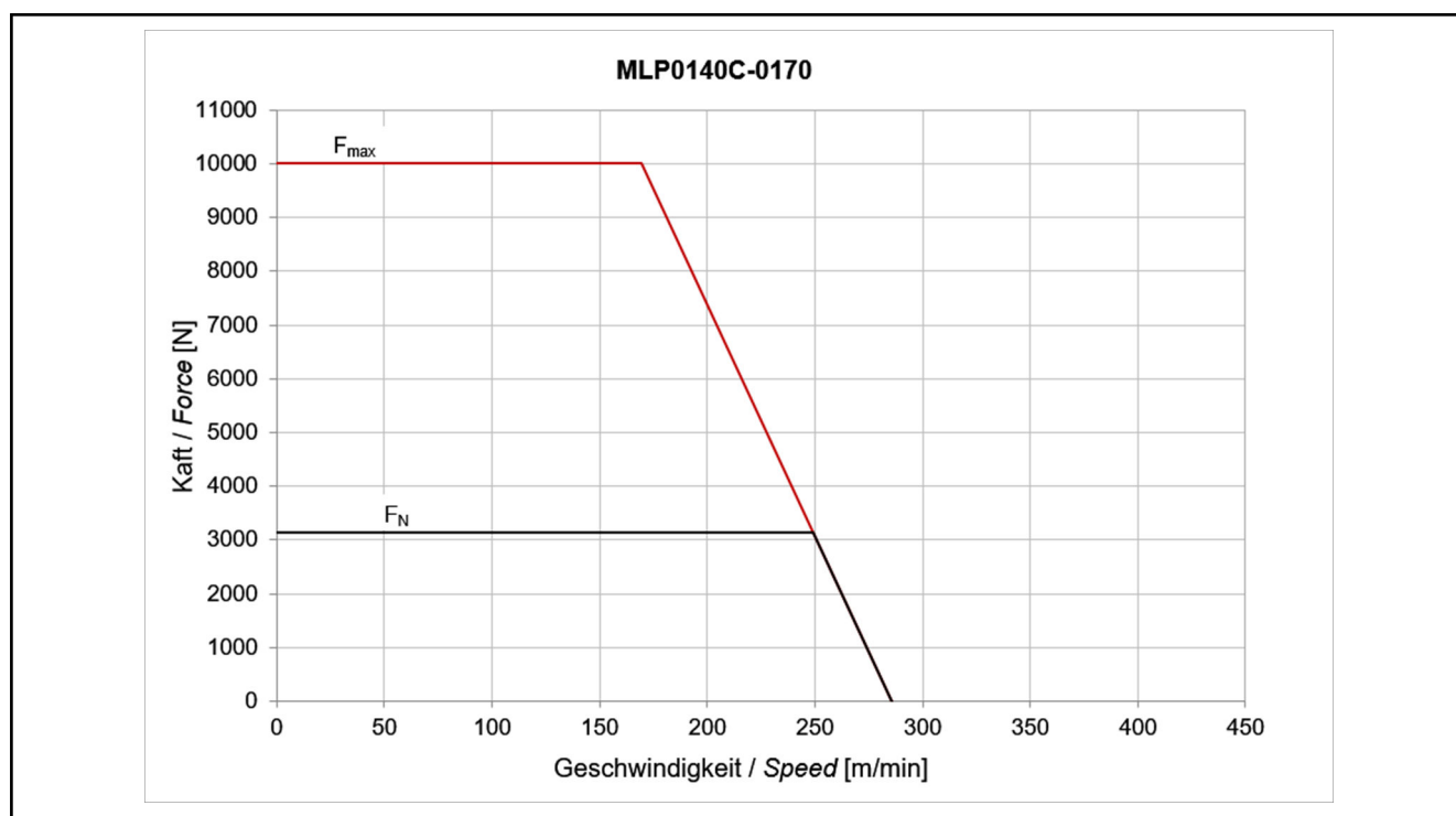
Fig. 4-45: Motor characteristic curves MLP140C-0170
