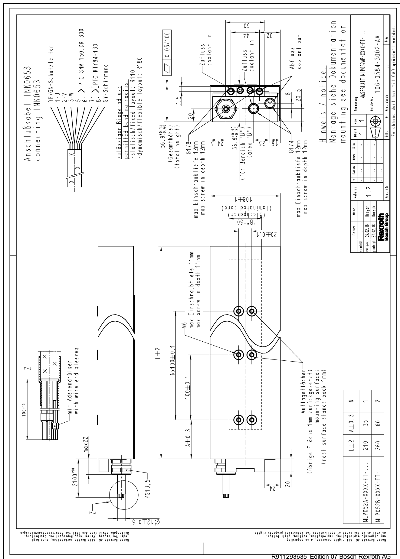
Fig. 5-5: Primary part MLP052 with thermo encapsulation
