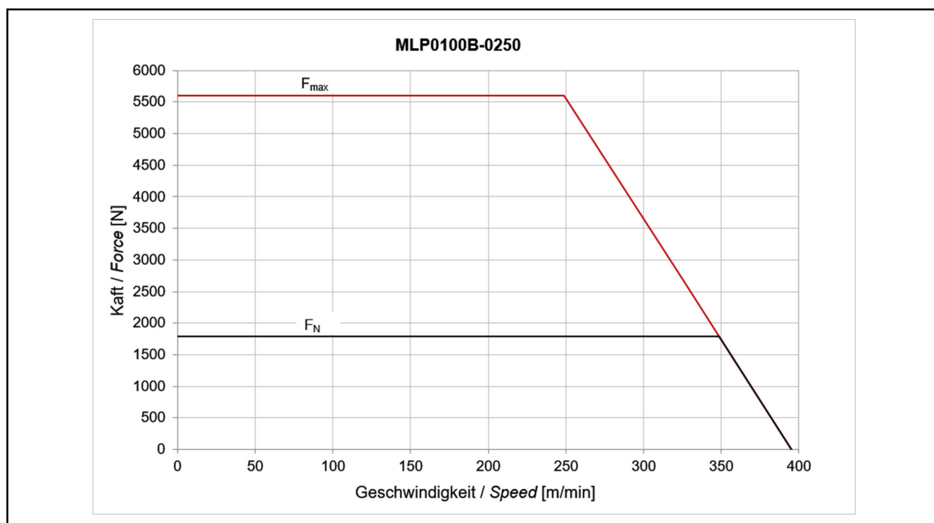
Fig. 4-30: Motor characteristic curves MLP100B-0250
