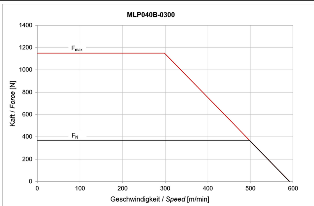
Fig. 4-7: Motor characteristic curve MLP040B-0300
