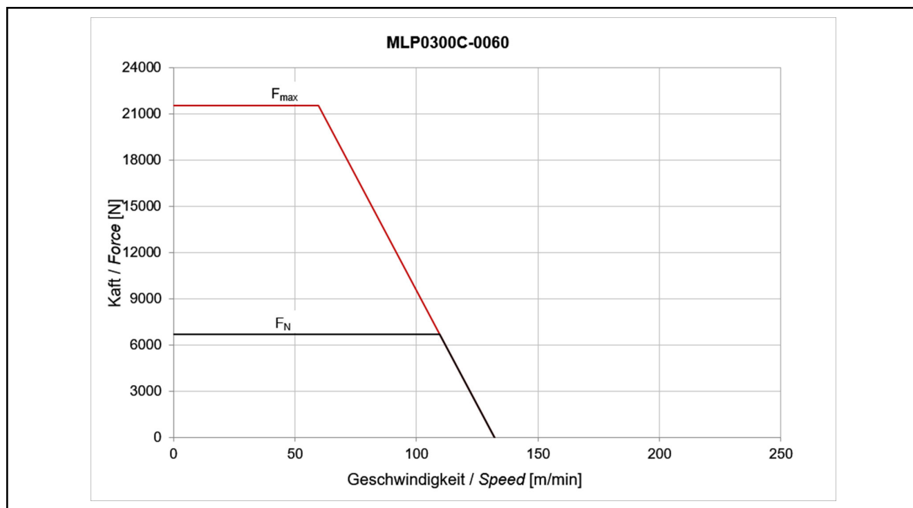
Fig. 4-70: Motor characteristic curve MLP300C-0060
