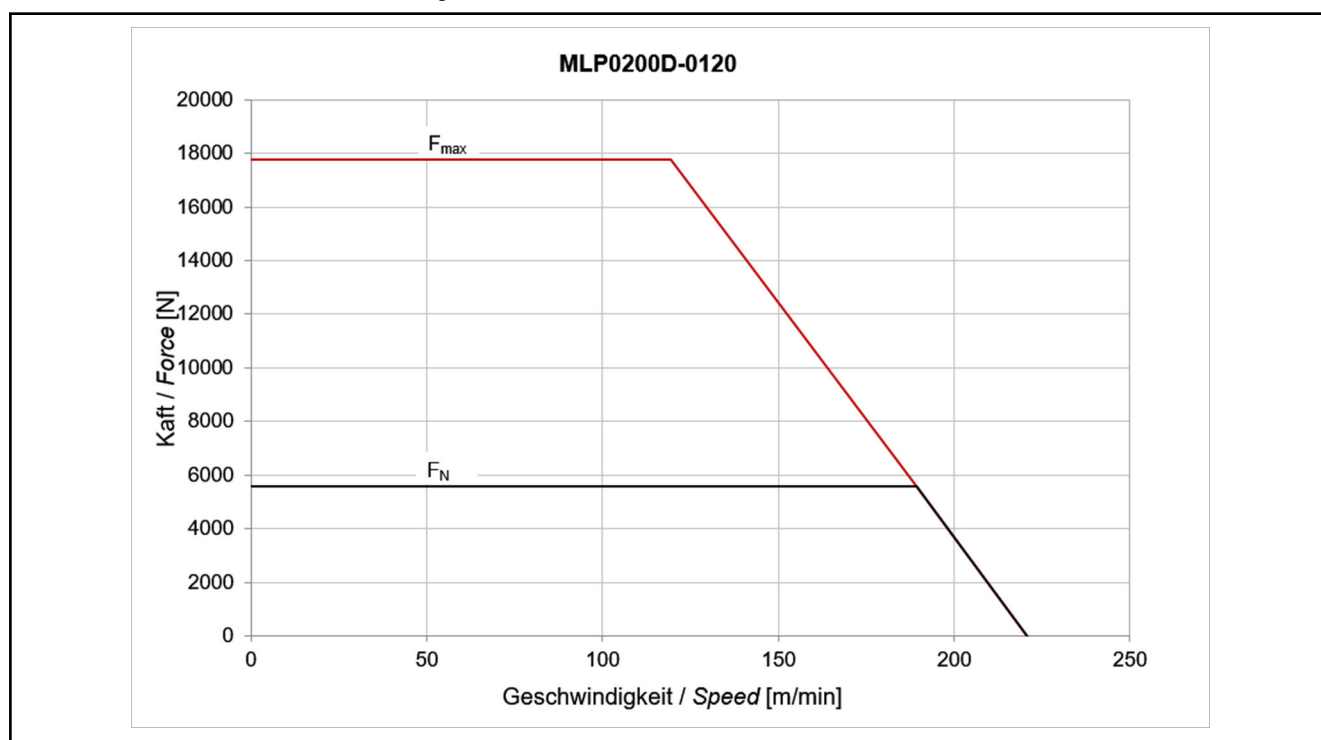
Fig. 4-61: Motor characteristic curves MLP200D-0120
