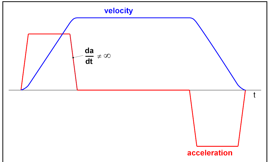
Fig. 9-66: Acceleration and speed with jerk limitation
