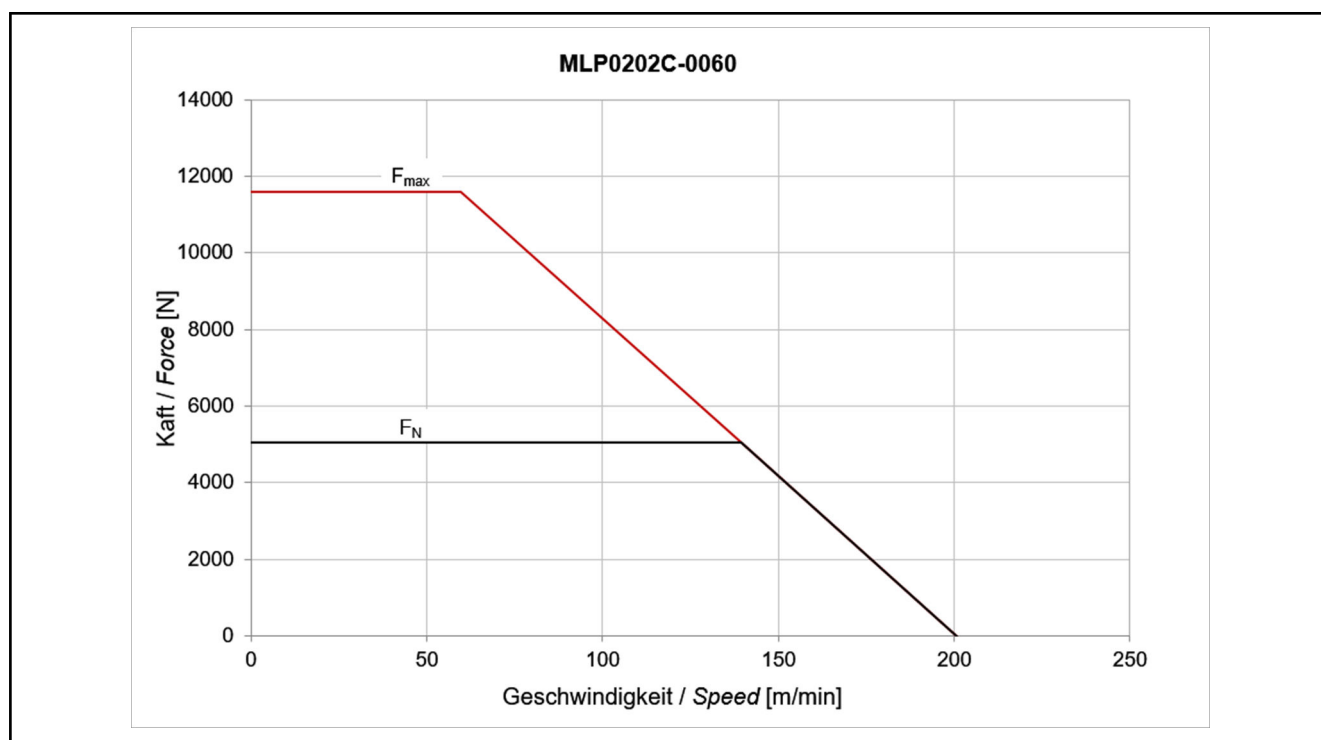
Fig. 4-64: Motor characteristic curve MLP0202C-0060
