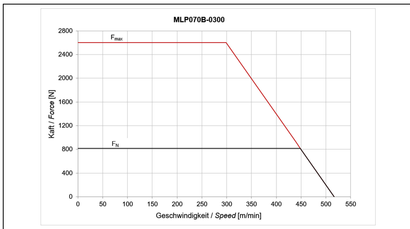
Fig. 4-17: Motor characteristic curves MLP070B-0300
