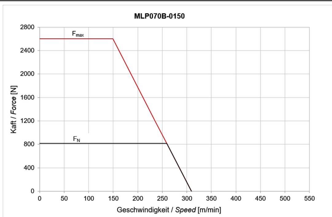
Fig. 4-15: Motor characteristic curves MLP070B-0150
