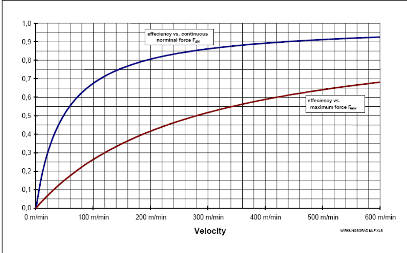
Fig. 10-30: Efficiency via velocity for MLF synchronous linear motors
