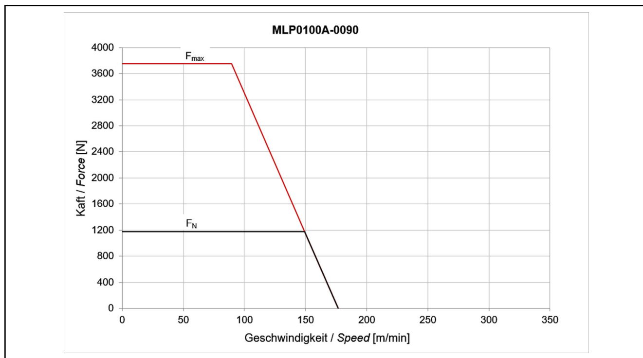
Fig. 4-23: Motor characteristic curve MLP100A-0090
