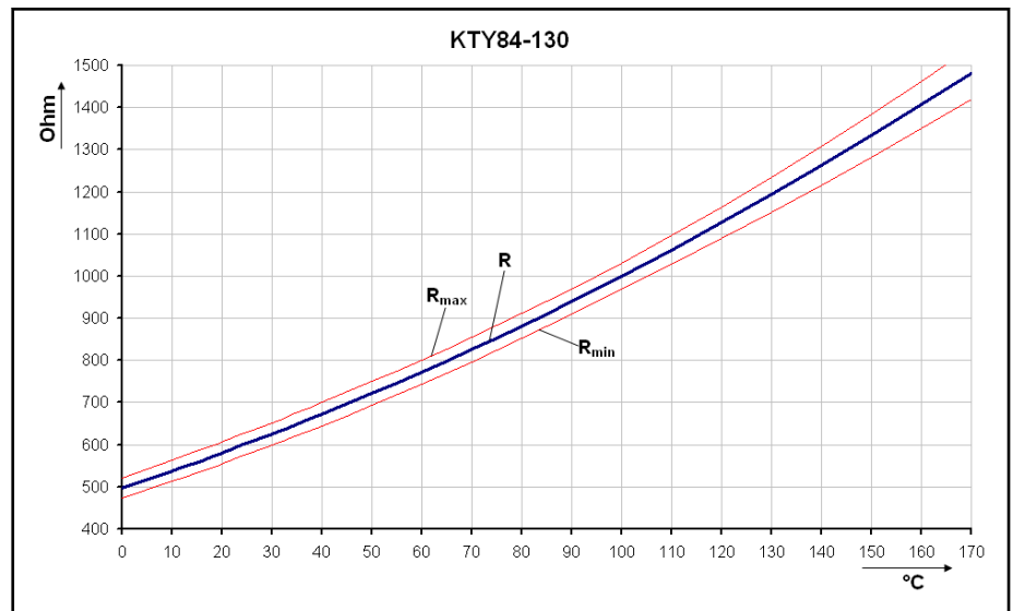
Fig. 9-32: Characteristic of temperature measurement sensor KTY84-130 (PTC)
