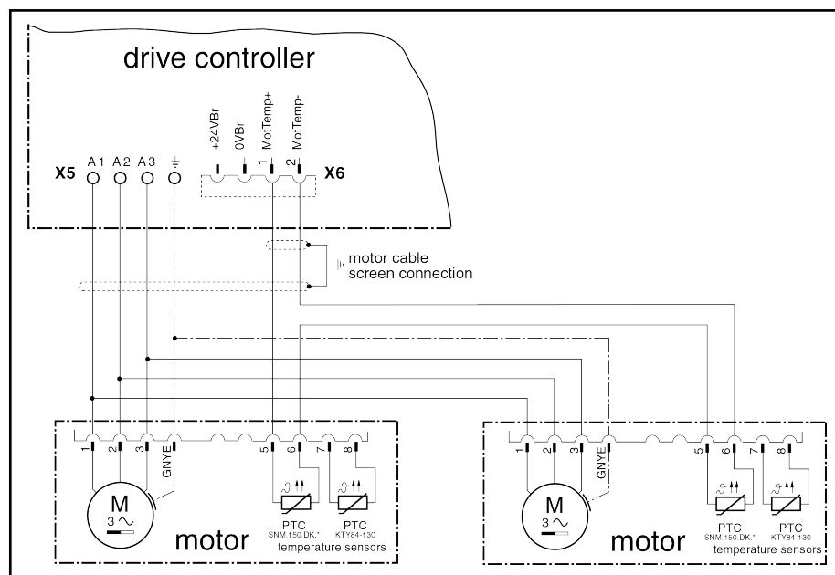
Fig. 8-10: Connection on drive controller - parallel connection primary part
