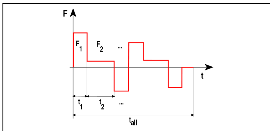
Fig. 10-3: Determining feed forces
