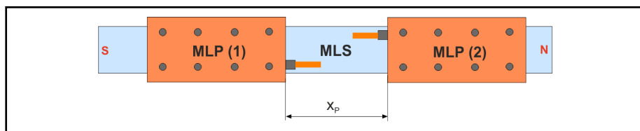
Fig. 9-47: Variant 2: Arrangement of primary parts behind each other with cable outlets in opposite directions
