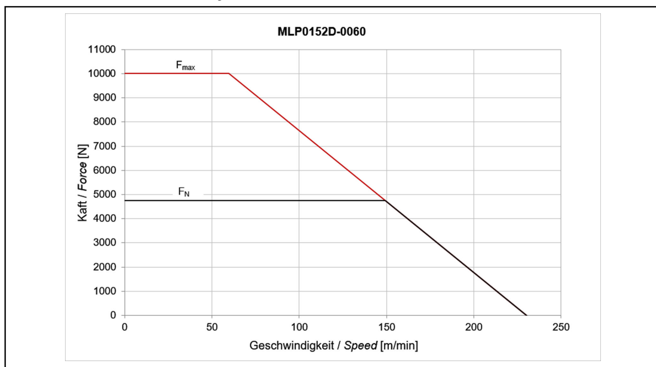
Fig. 4-50: Motor characteristic curve MLP152D-0060
