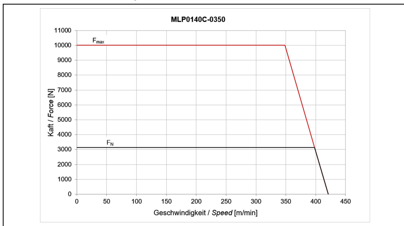
Fig. 4-46: Motor characteristic curves MLP140C-0350
