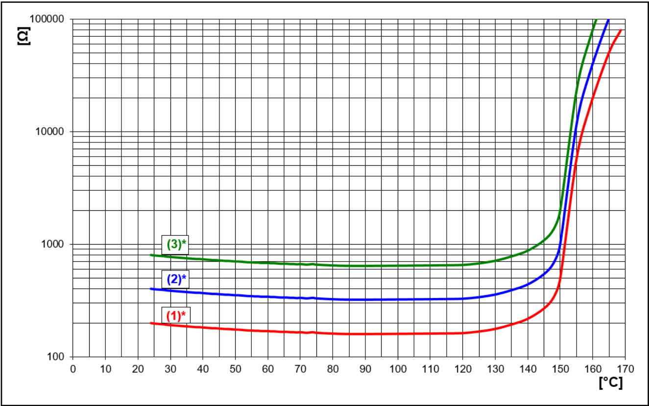
1 2 (3) 1x SNM.150.DK at 1x MLP 2x SNM.150.DK at 2x MLP 4x SNM.150.DK at 4x MLP Fig. 9-31: Characteristic of temperature sensors for motor protection (SNM150.DK)
