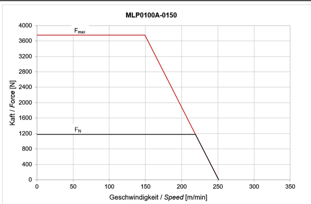
Fig. 4-25: Motor characteristic curves MLP100A-0150
