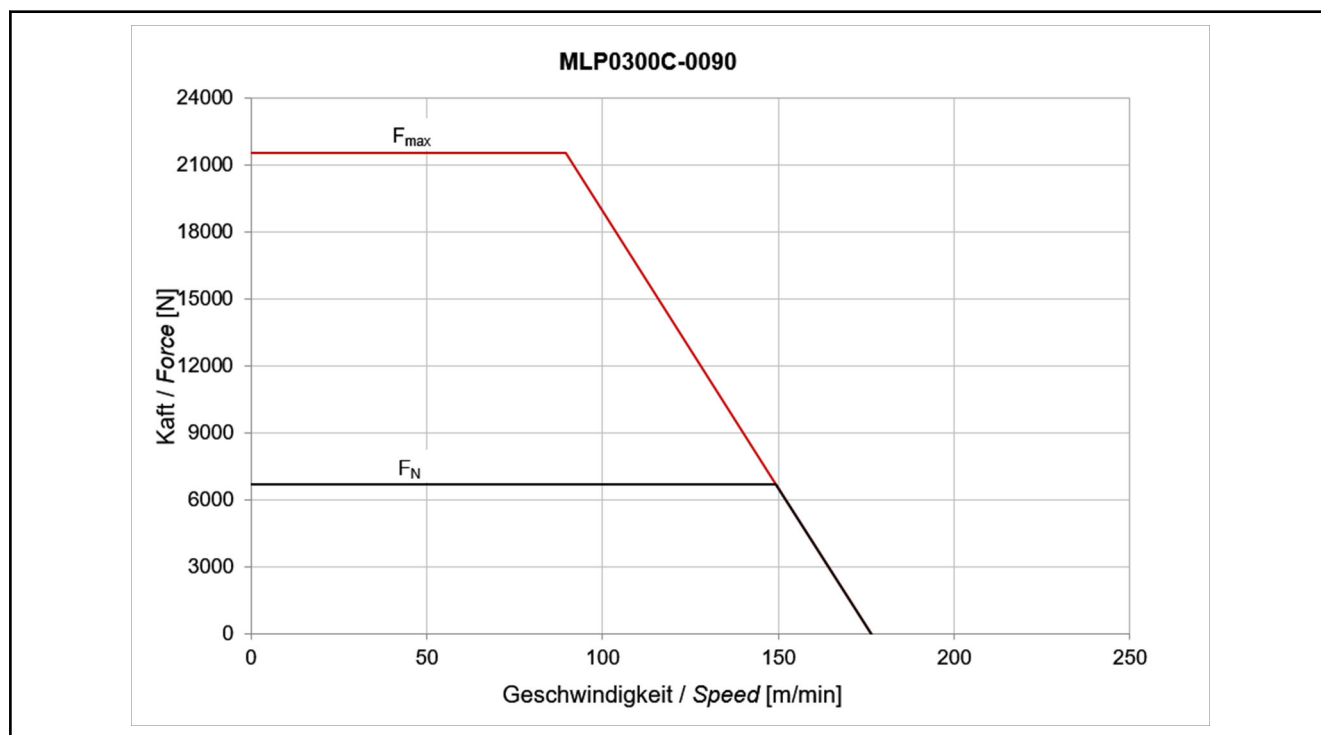
Fig. 4-71: Motor characteristic curves MLP300C-0090
