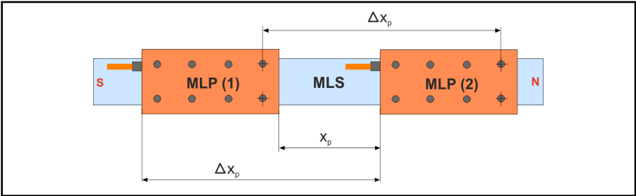
Fig. 9-42: Arrangement of the primary parts behind each other and cable outlets in the same direction
