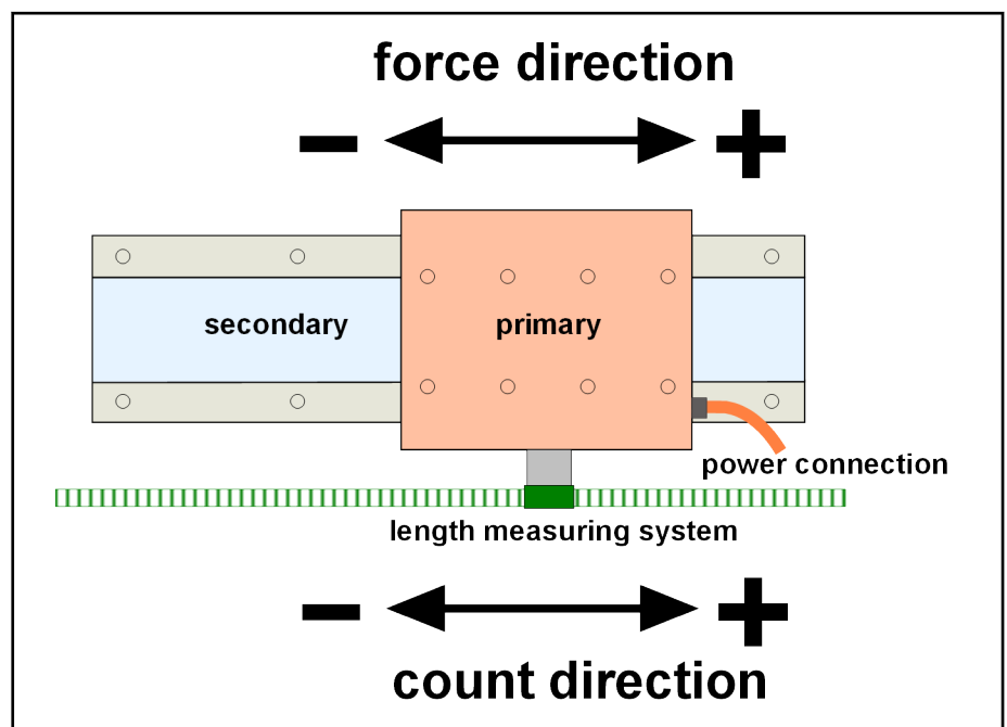
Fig. 13-3: Effective direction of the motor force = Counting direction of the length measuring system
