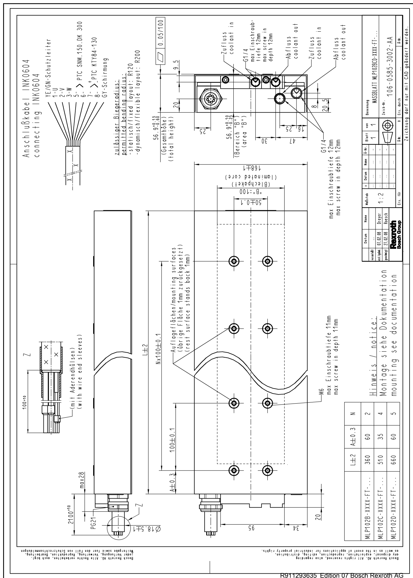
Fig. 5-13: Primary part MLP102 with thermo encapsulation
