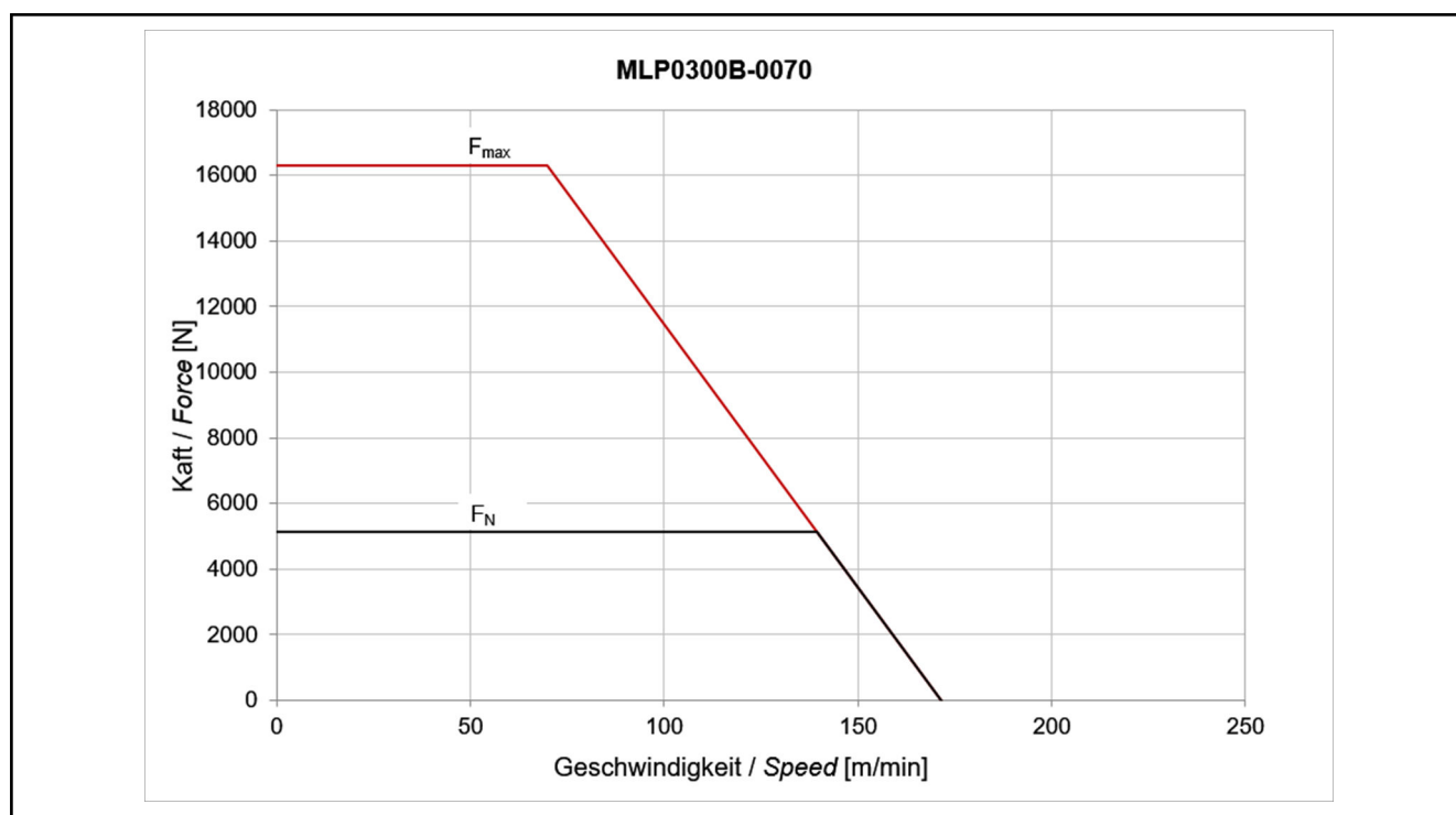
Fig. 4-68: Motor characteristic curve MLP300B-0070
