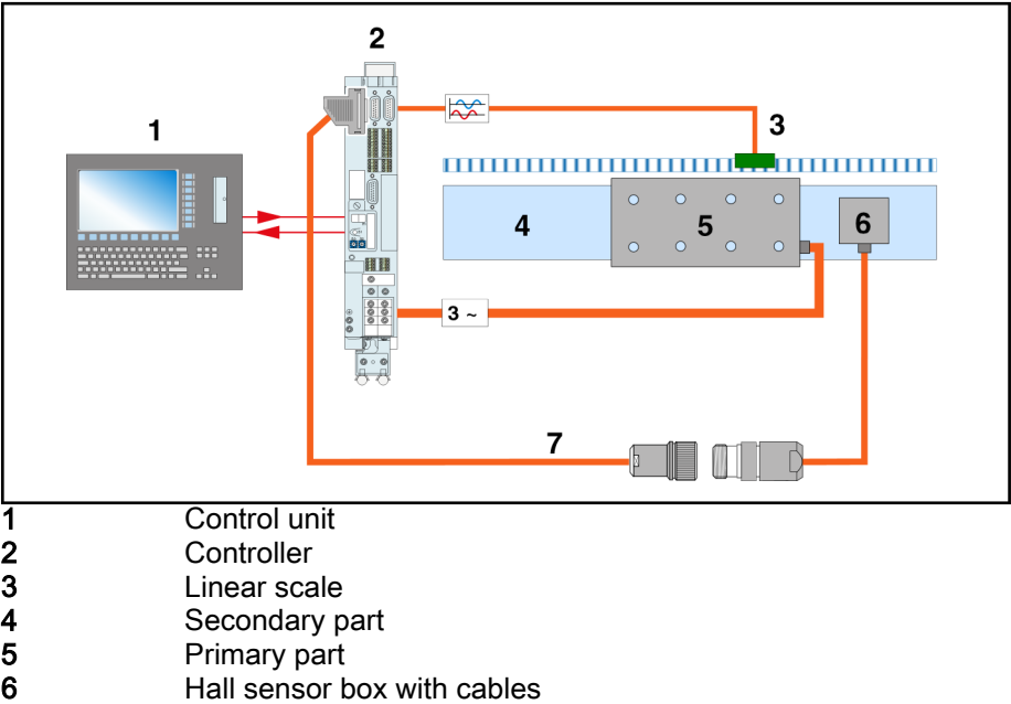
Fig. 7-2: Schematic setup MLF with a Hall sensor box
