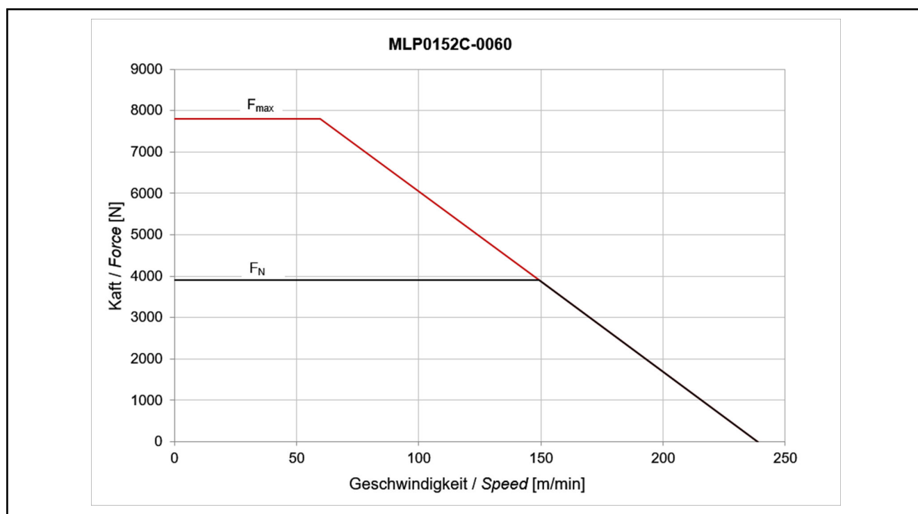
Fig. 4-49: Motor characteristic curve MLP152C-0060
