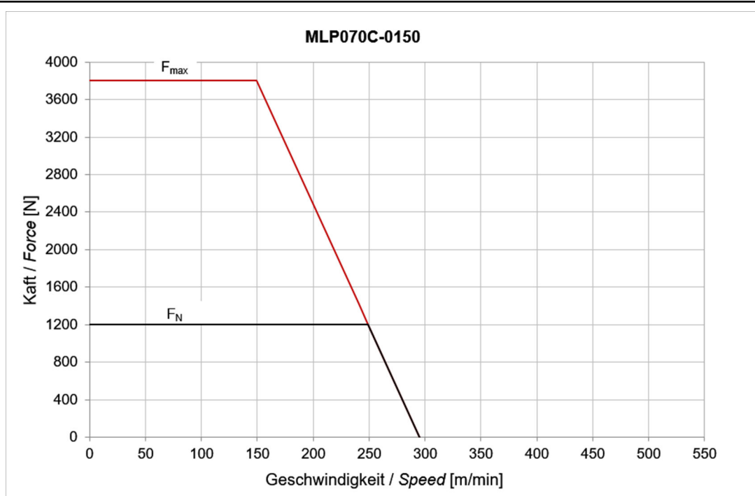
Fig. 4-20: Motor characteristic curves MLP070C-0150
