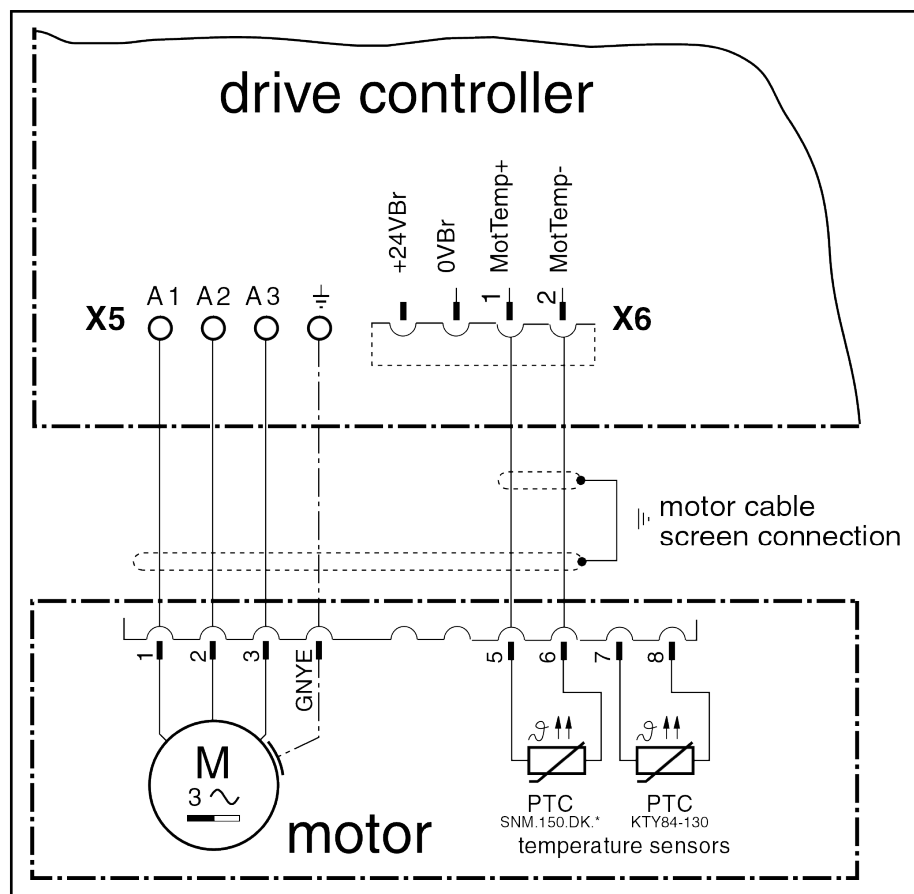
Fig. 8-9: Connection on drive controller - single arrangement primary part
