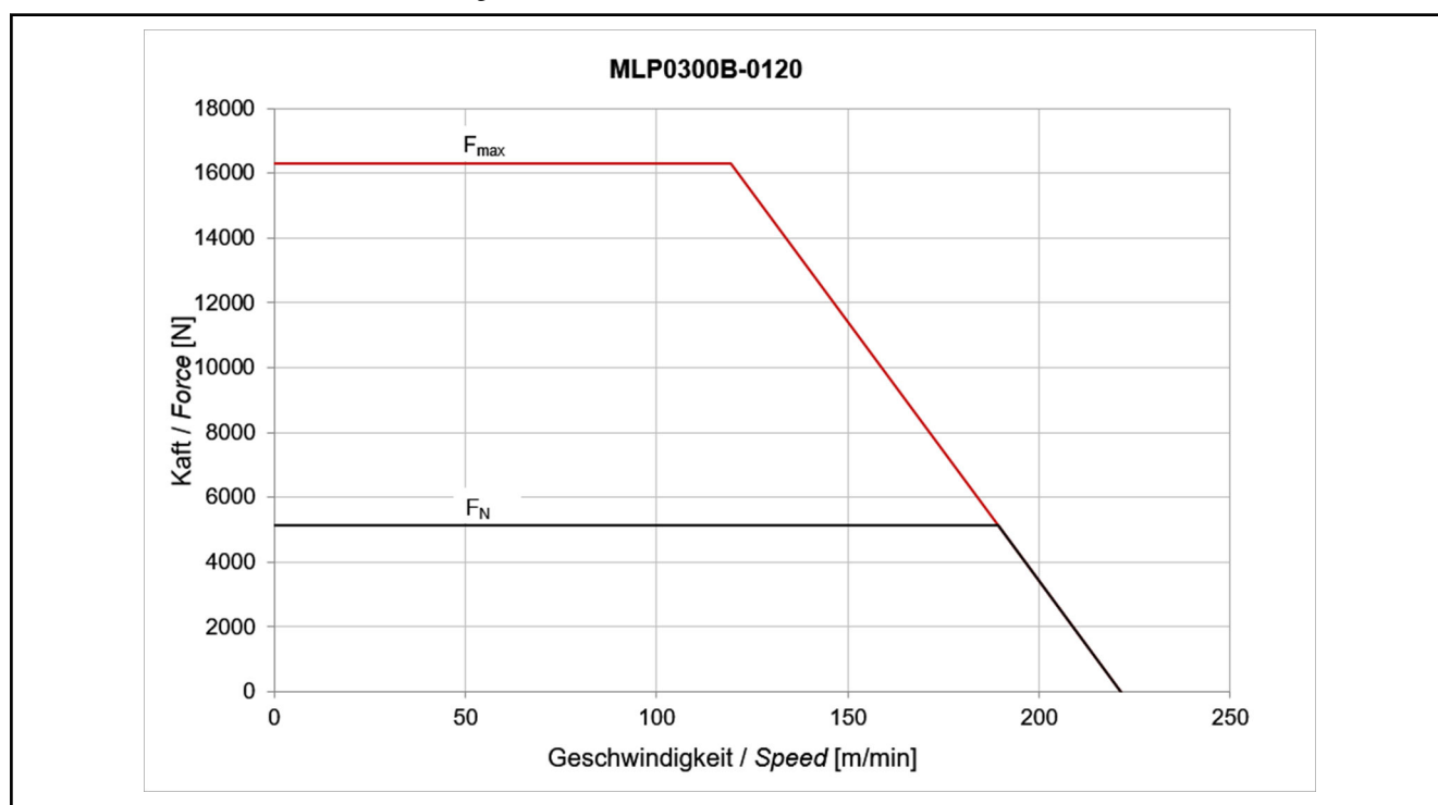
Fig. 4-69: Motor characteristic curves MLP300B-0120
