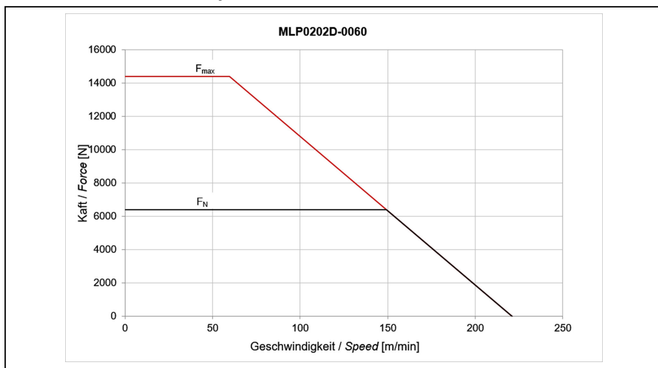
Fig. 4-65: Motor characteristic curve MLP0202D-0060
