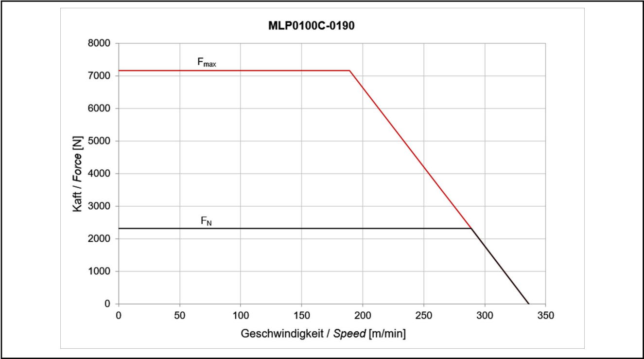
Fig. 4-33: Motor characteristic curves MLP100C-0190
