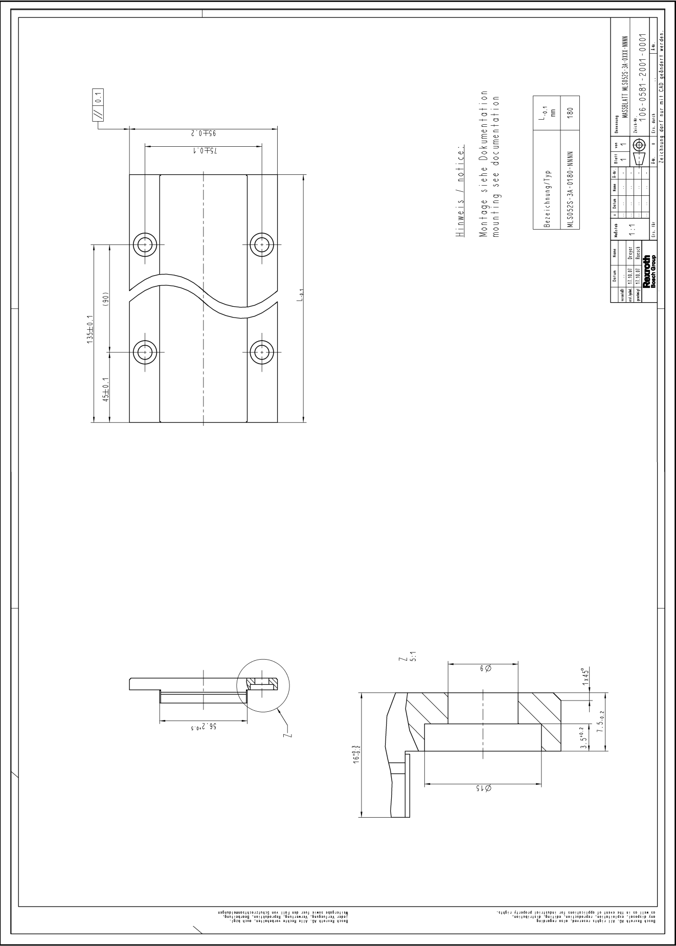
Bosch Rexroth AG R911293635_Edition 07 Fig. 5-6: Secondary part MLS052
