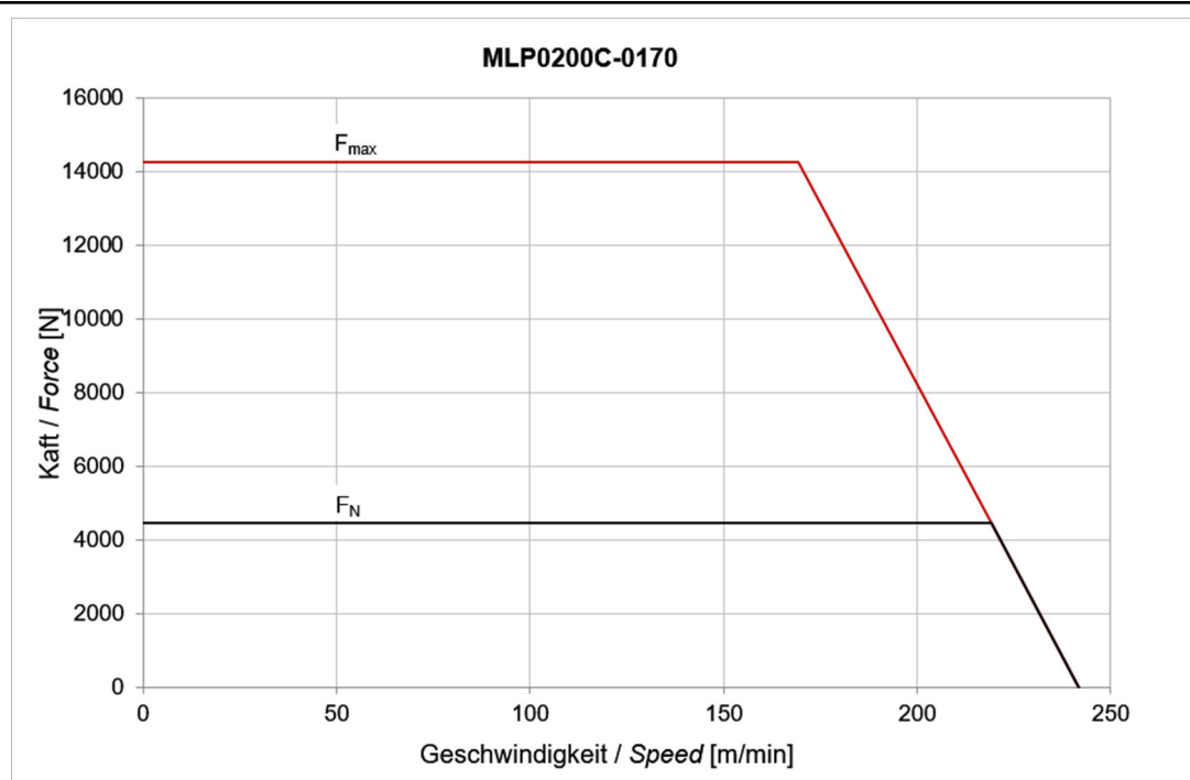
Fig. 4-57: Motor characteristic curves MLP200C-0170
