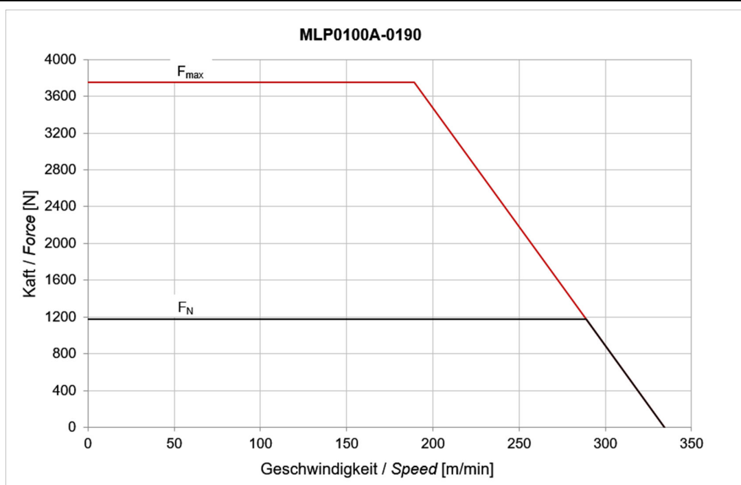
Fig. 4-26: Motor characteristic curves MLP100A-0190
