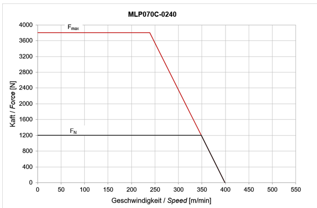
Fig. 4-21: Motor characteristic curves MLP070C-0240
