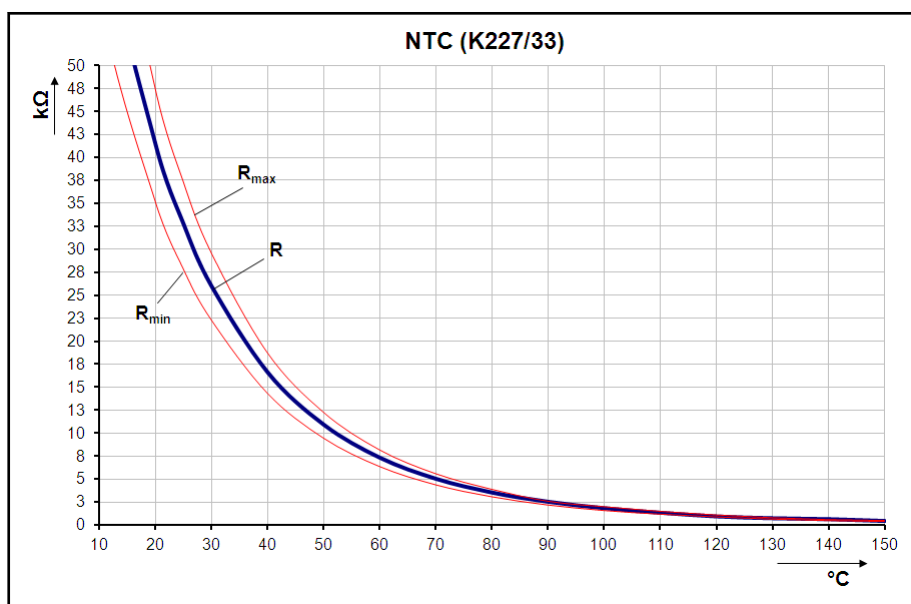
Fig. 9-6: Characteristic thermistor (NTC)
