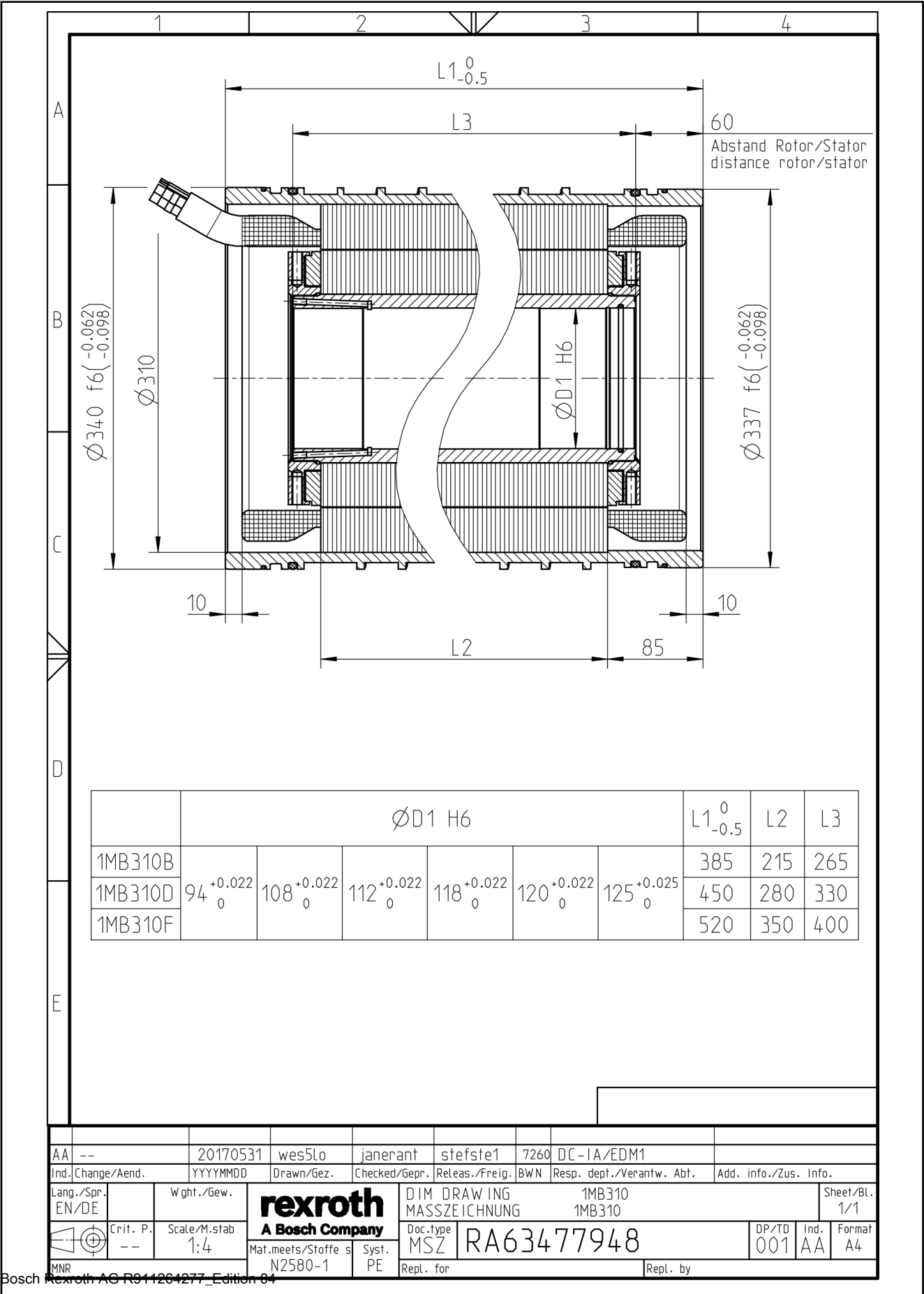
Fig. 5-41: Dimension sheets 1MB310
