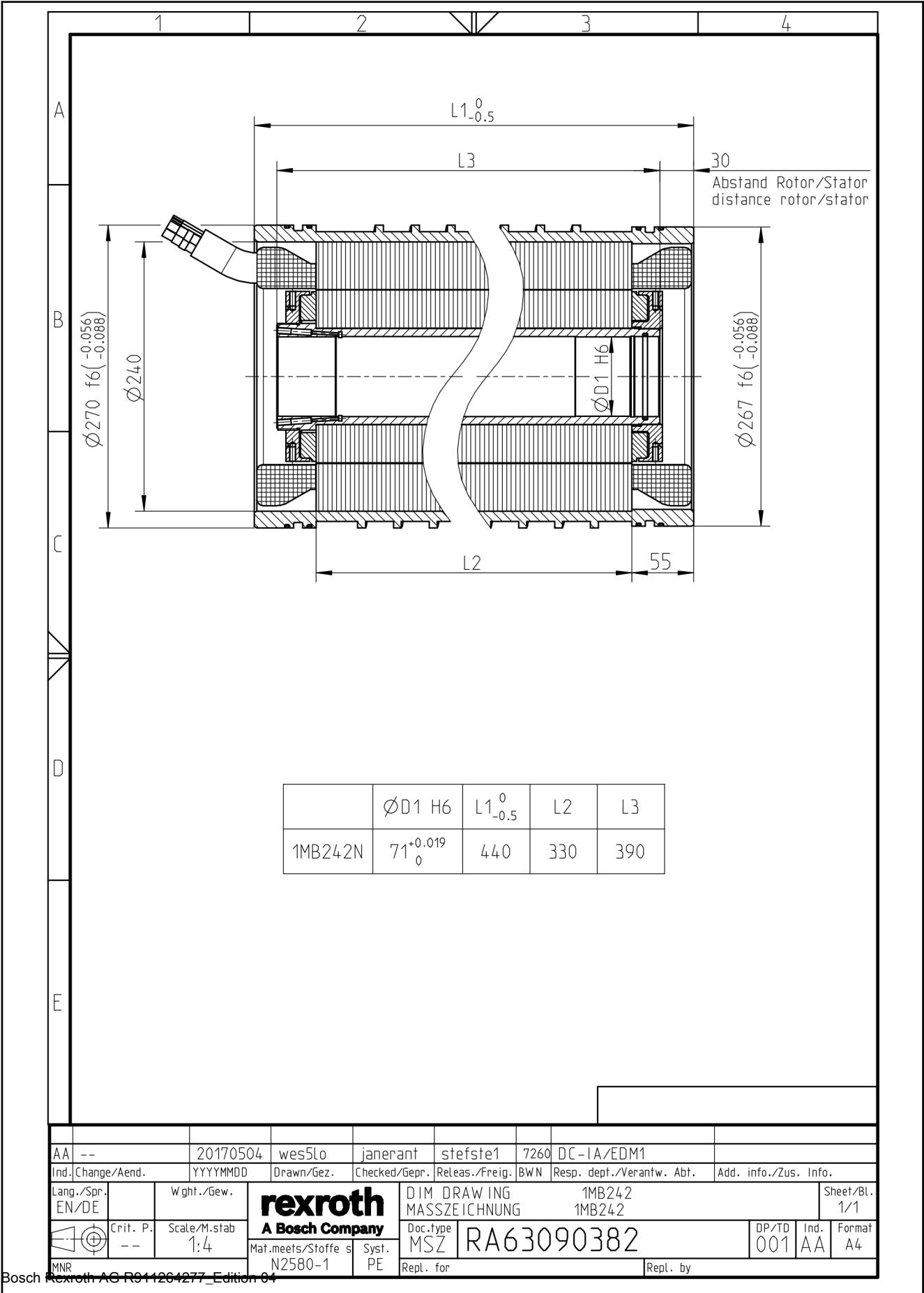
Fig. 5-31: Dimension sheet 1MB242
