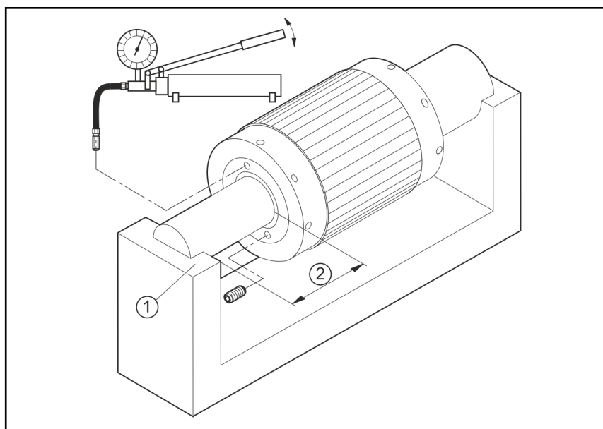
Fig. 11-14: Example of a fixture for disassembly
