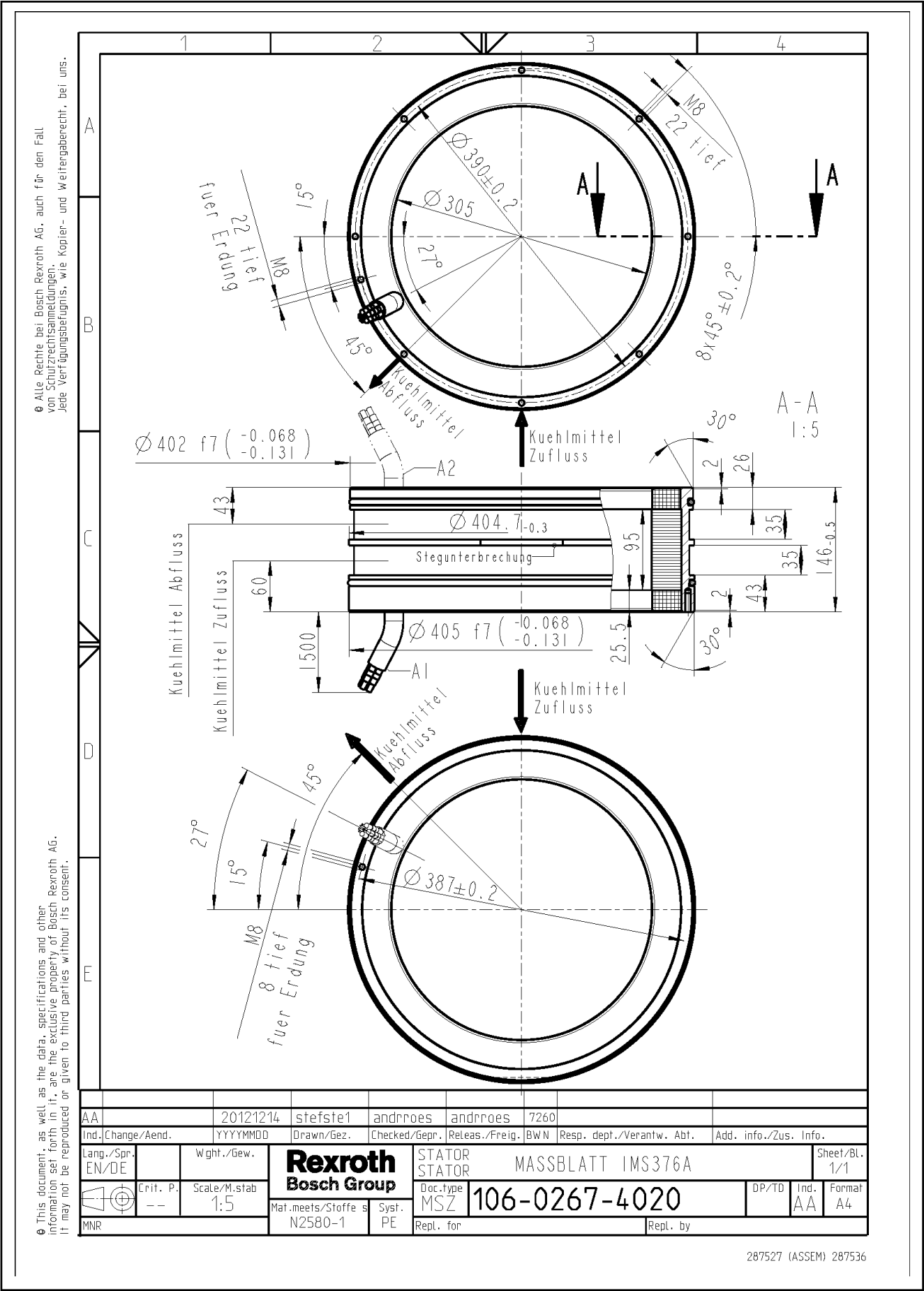
Bosch Rexroth AG R911264277_Edition 04 Fig. 5-53: Dimension sheet 1MS376
