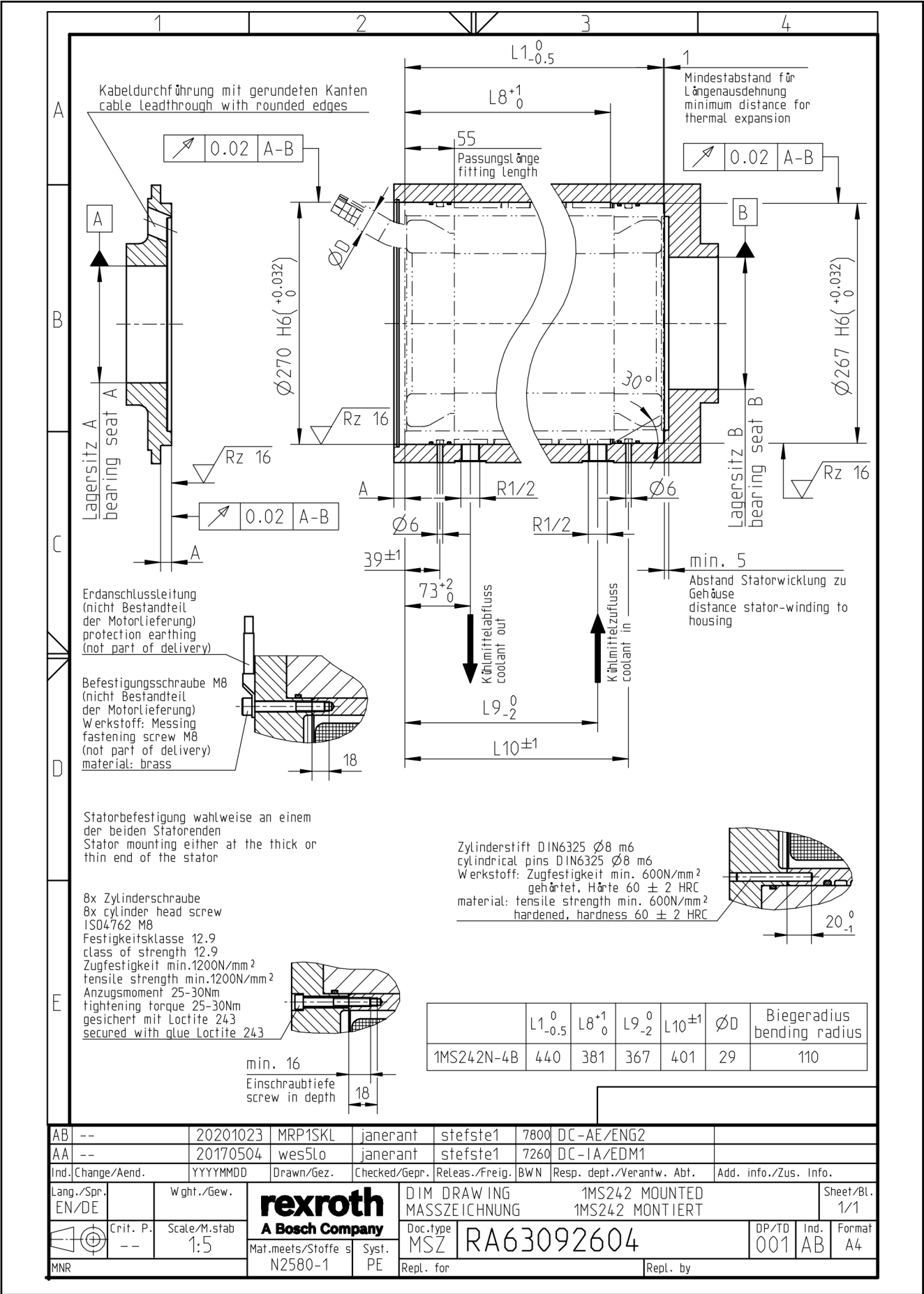
Bosch Rexroth AG R911264277_Edition 04 Fig. 5-35: Dimension sheet 1MS242, mounted
