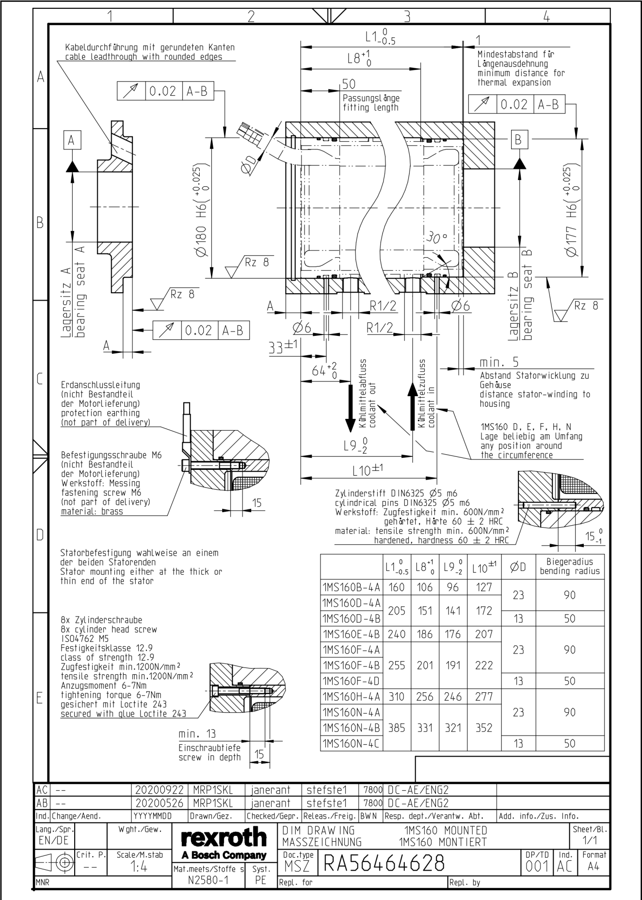
Bosch Rexroth AG R911264277_Edition 04 Fig. 5-15: Dimension sheet 1MS160, mounted
