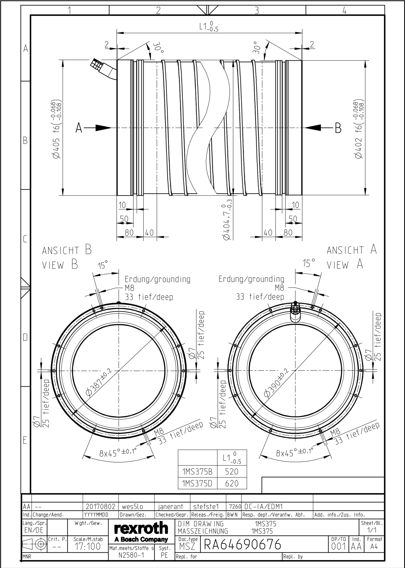
Bosch Rexroth AG R911264277_Edition 04 Fig. 5-49: Dimension sheet 1MS375
