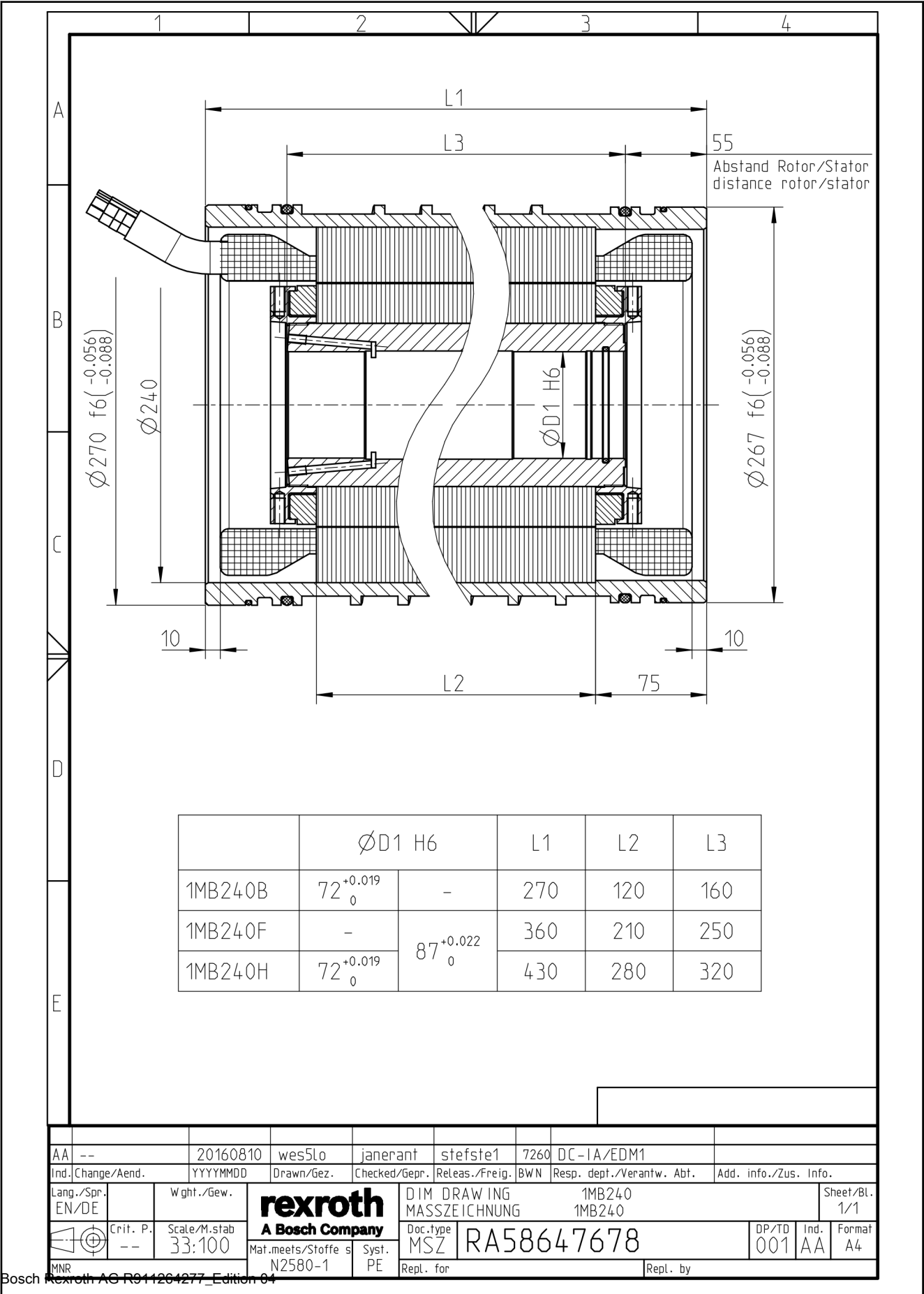
Fig. 5-21: Dimension sheet 1MB240
