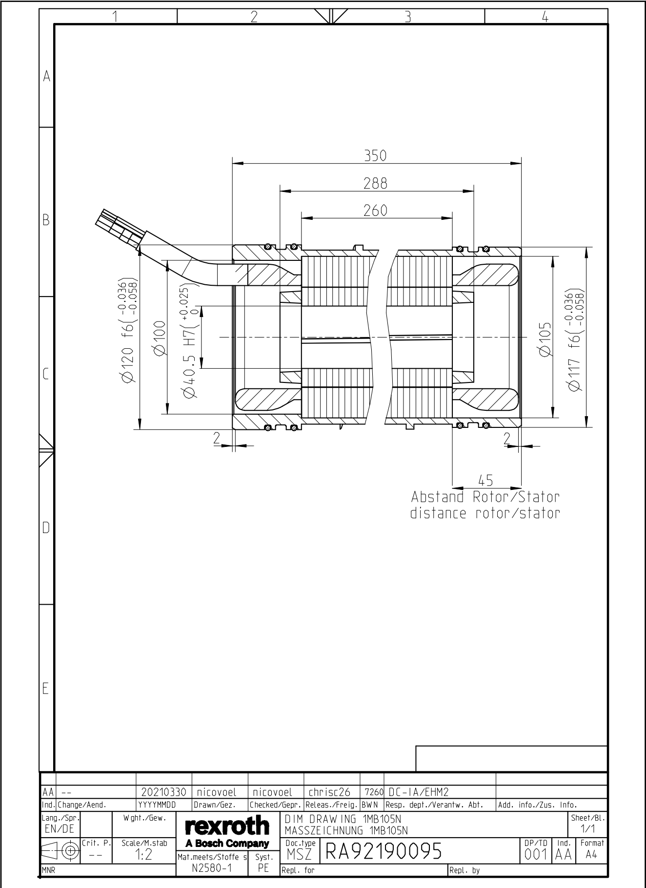
Bosch Rexroth AG R911264277_Edition 04 Fig. 5-1: 1MB105 Dimension sheets
