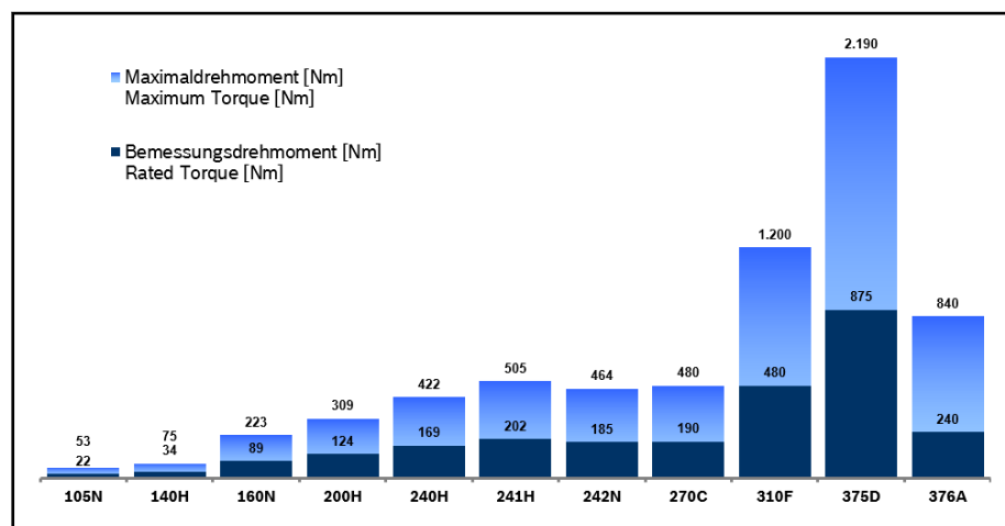
Fig. 1-2: Size and power grading
