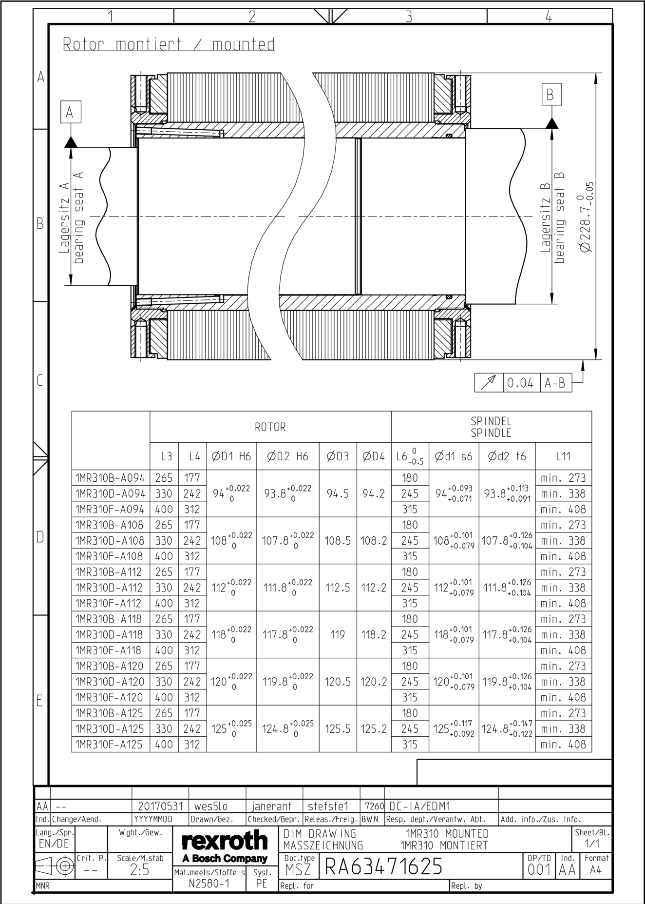
Bosch Rexroth AG R911264277_Edition 04 Fig. 5-43: Dimension sheet 1MR310, mounted
