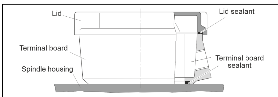
Fig. 11-22: Sealings on the terminal box
