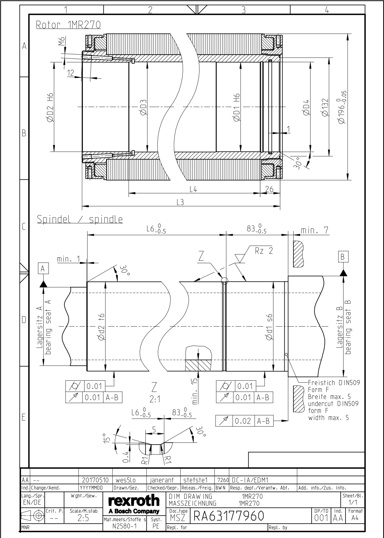
Bosch Rexroth AG R911264277_Edition 04 Fig. 5-37: Dimension sheet 1MR270
