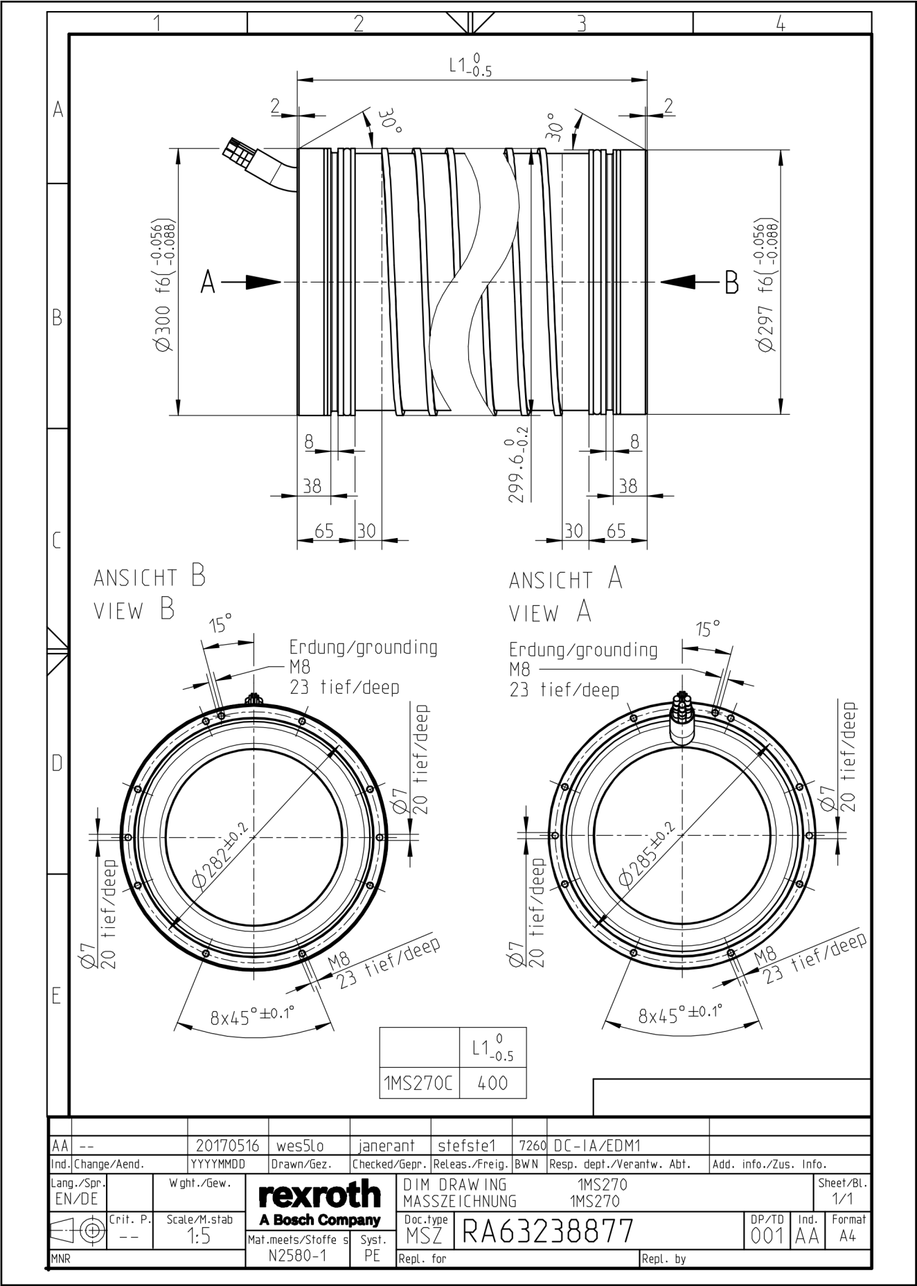
Bosch Rexroth AG R911264277_Edition 04 Fig. 5-39: Dimension sheet 1MS270
