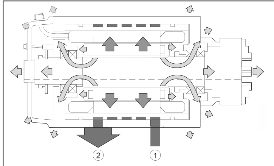
Fig. 9-2: Heat flows in the motor spindle
