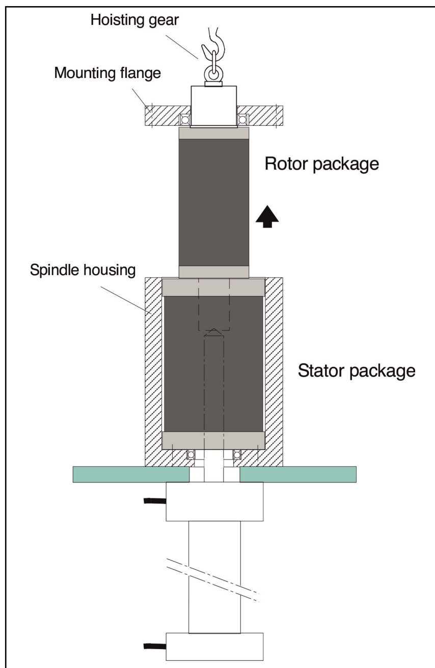
Fig. 11-15: Motor spindle disassembly
