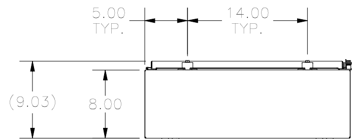
BOTTOM VIEW
