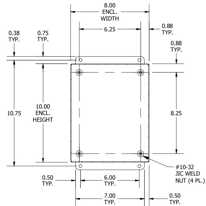
SECTION K-K (INSIDE BACK OF ENCLOSURE)
