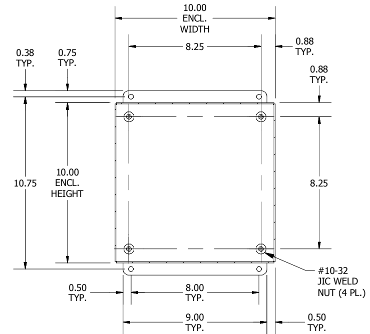
SECTION K-K (INSIDE BACK OF ENCLOSURE)
