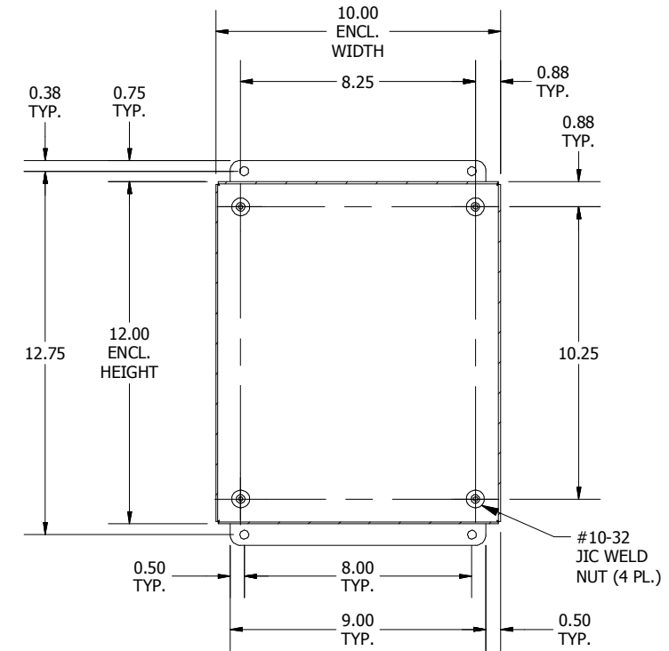
SECTION K-K (INSIDE BACK OF ENCLOSURE)
