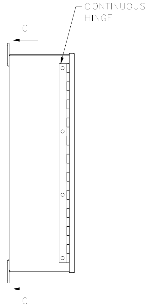
LEFT VIEW
