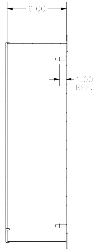
SECTION B-B SIDE VIEW
